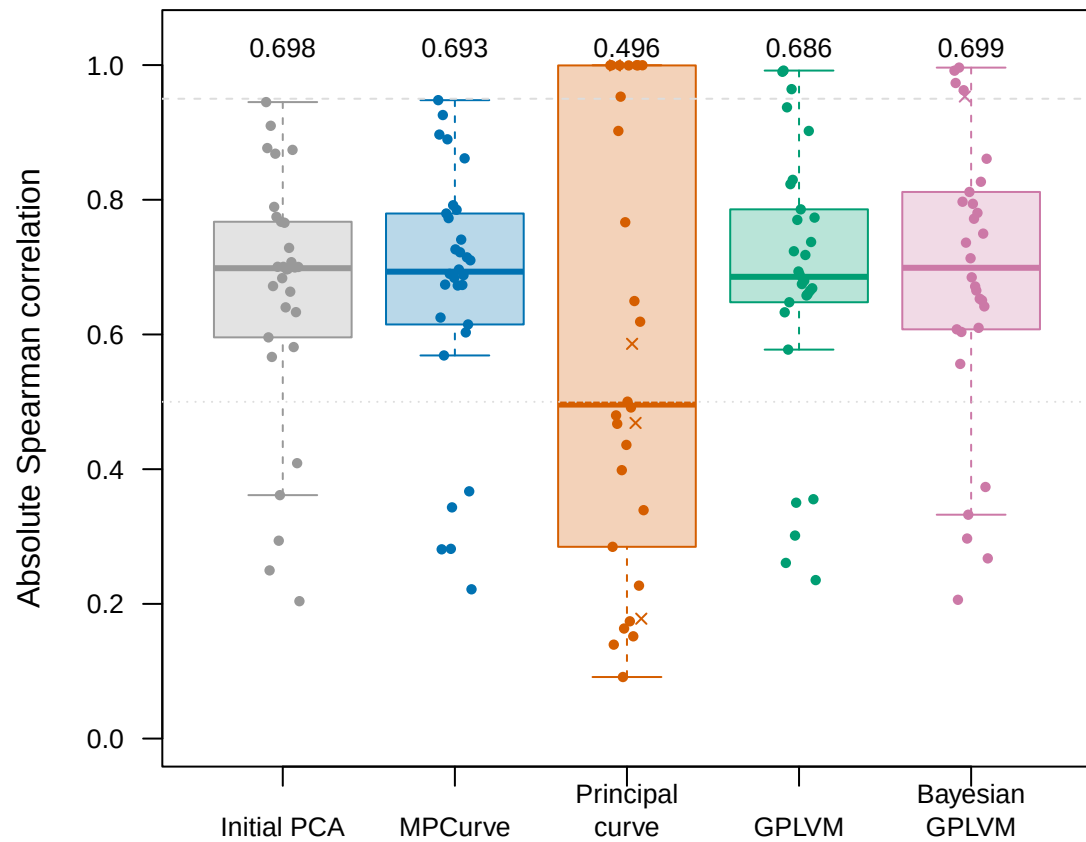
P = 50 | Low noise (SNR 16)
