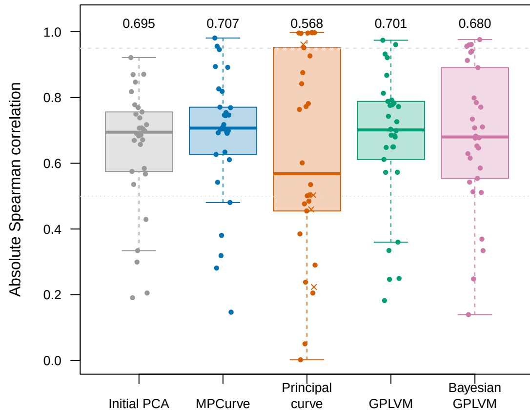
P = 50 | High noise (SNR 1)
