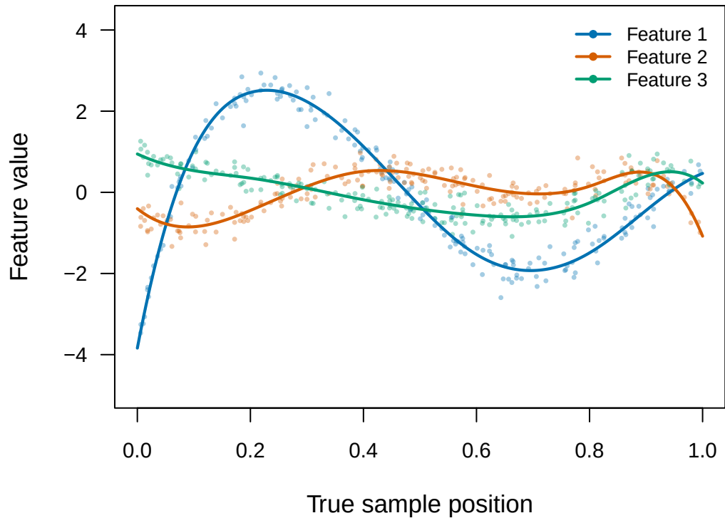
Simpler: low noise (SD 0.25)
