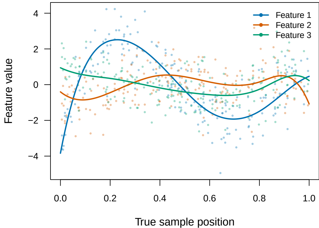
Challenging: high noise (SD 1)
