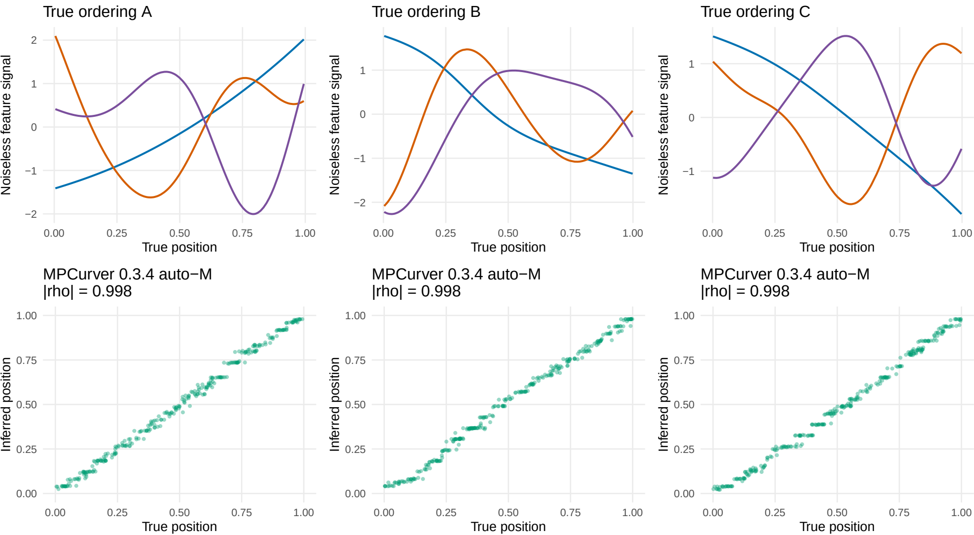
Top row: one monotone anchor (blue) and two nonmonotone smooth trajectories per true ordering. Bottom row: one-to-one matched inferred positions, with reversal allowed.
