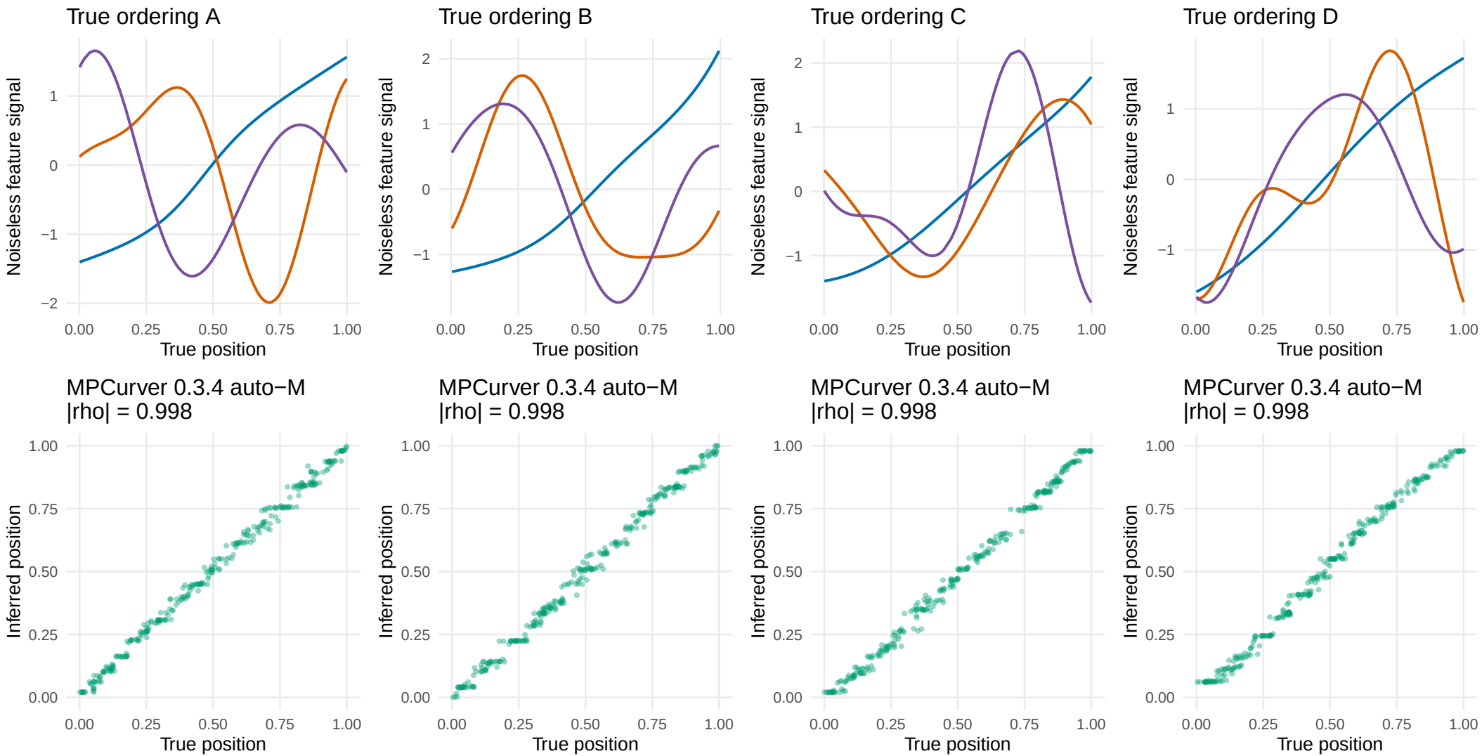
Top row: one monotone anchor (blue) and two nonmonotone smooth trajectories per true ordering. Bottom row: one-to-one matched inferred positions, with reversal allowed.
