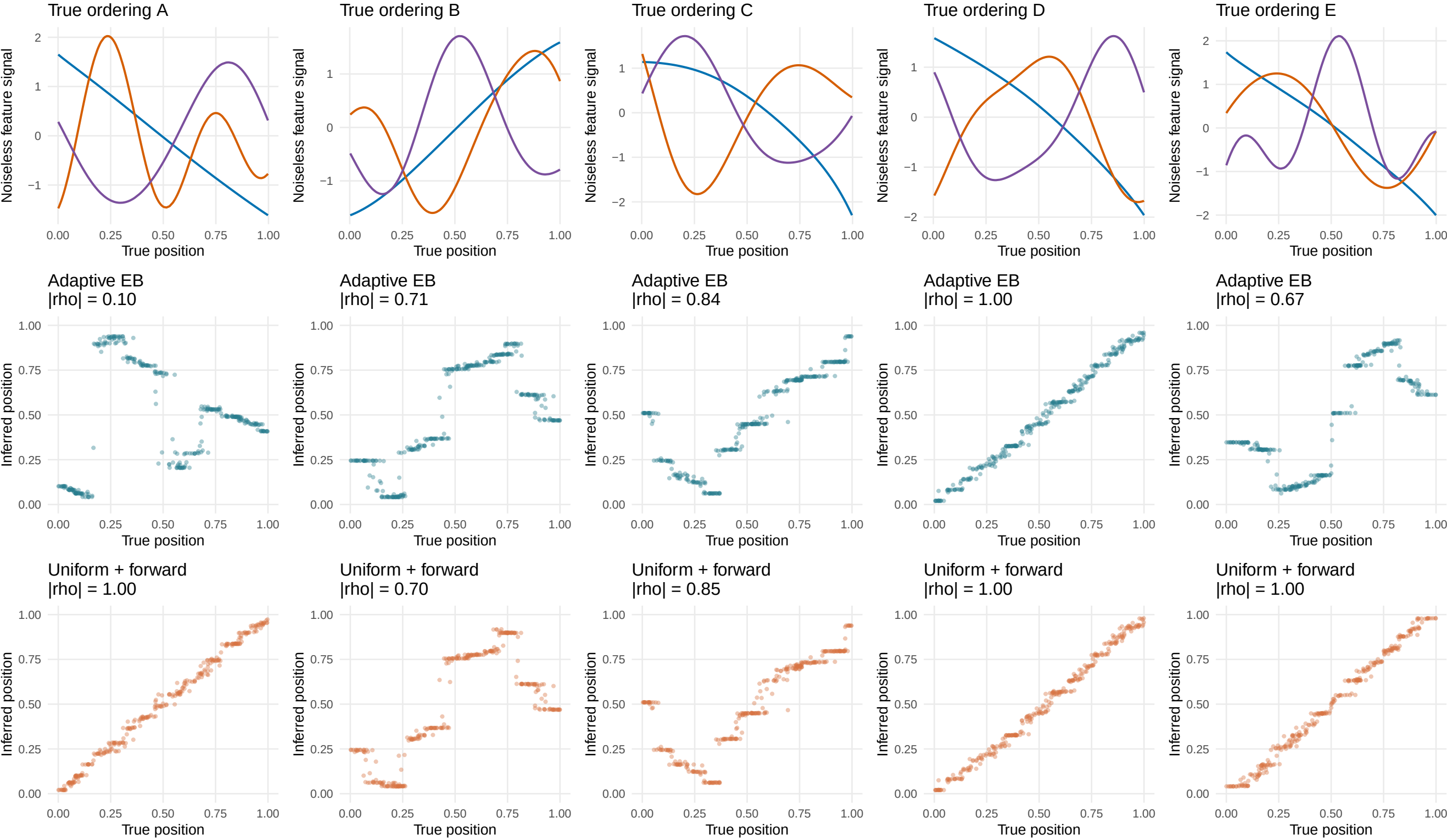
Top row: monotone anchor (blue) and two smooth trajectories (orange and purple) per true ordering. Other rows: one-to-one matches of occupied inferred orderings to truth, with reversal allowed; an unmatched true ordering has score zero.
