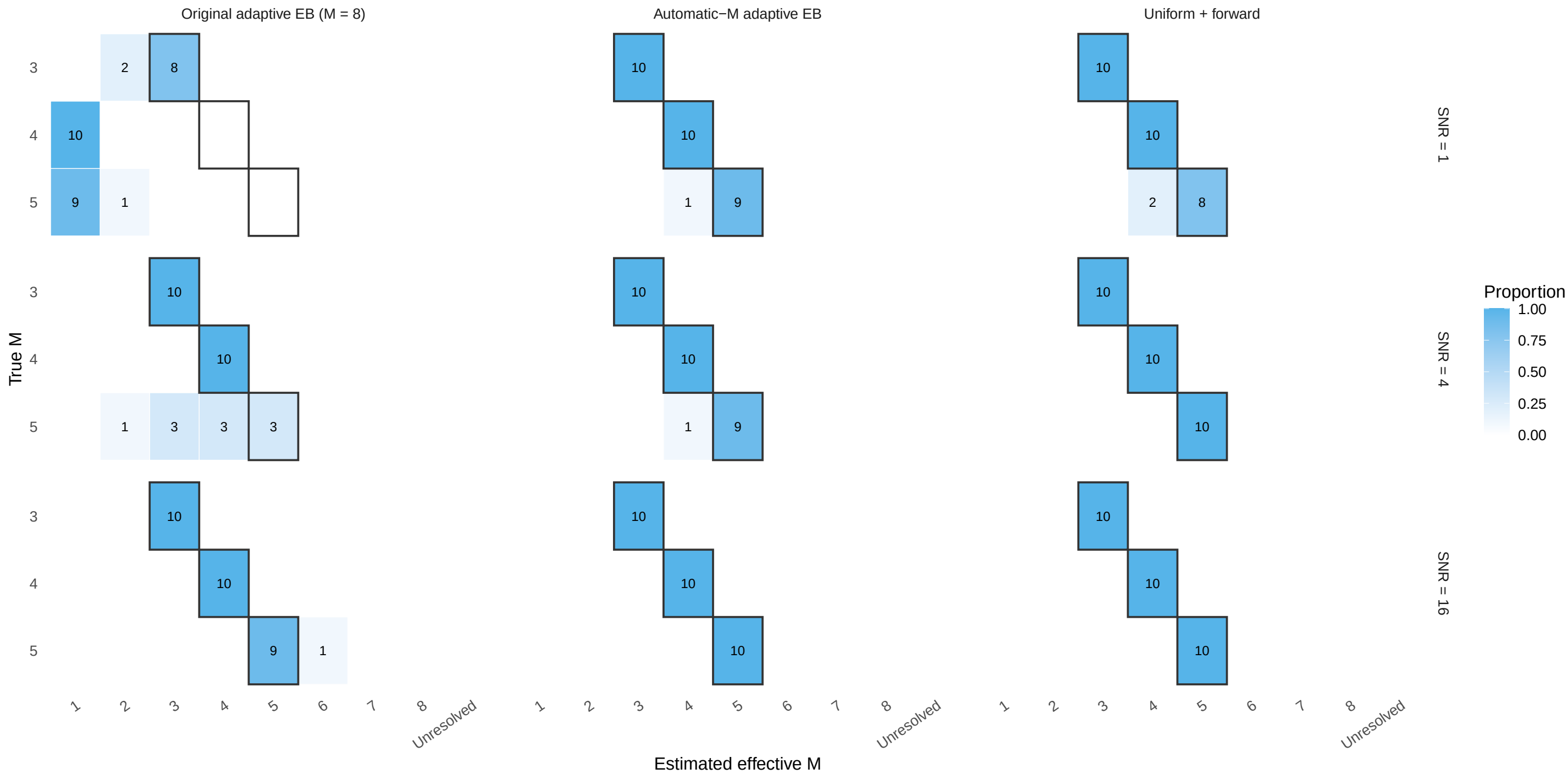
Distribution of estimated ordering counts Cell labels give counts out of 10; outlined cells recover the true M
