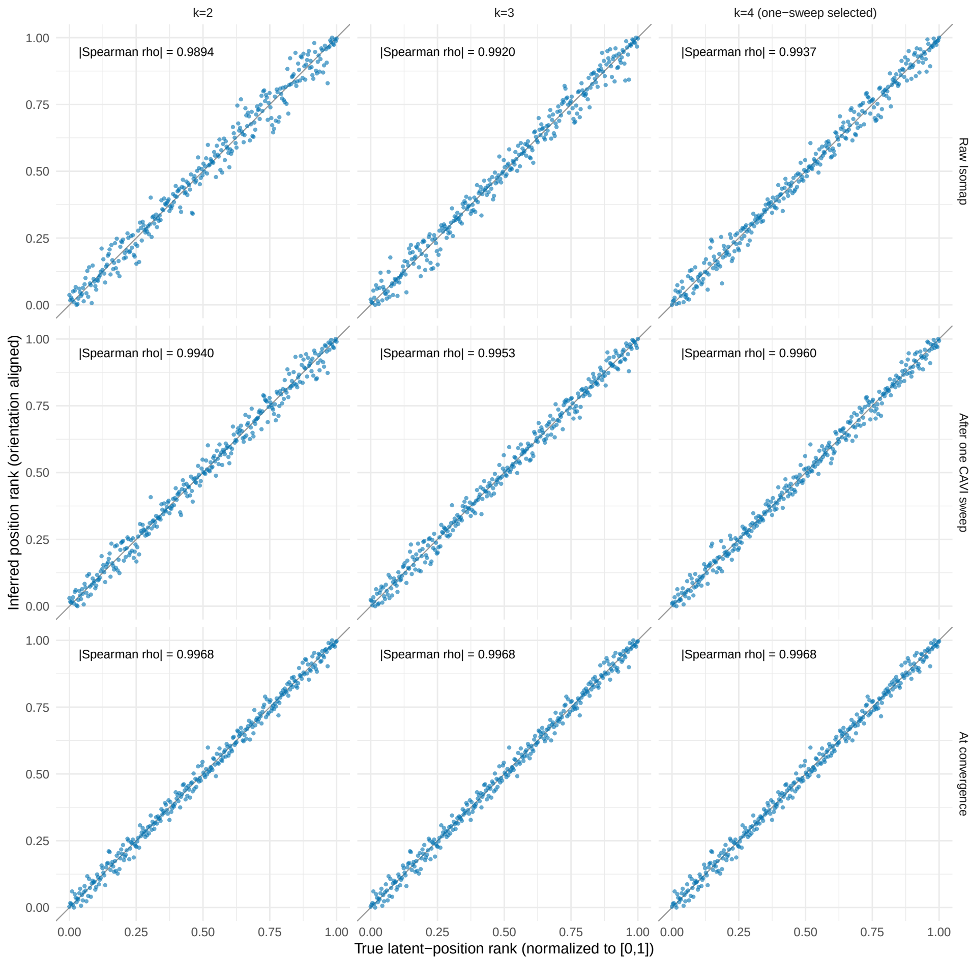
Figure 1. All 300 sample ranks under Isomap k=2,3,4 on the original 12-feature B group. Rows show raw Isomap, one MPCurve CAVI sweep, and continuation to convergence. The column marked selected has the highest one-sweep ELBO within [2,4]. Orientation is aligned using truth for display only; the gray diagonal is perfect rank recovery. All candidates use 50 position bins and identical fitting settings.
