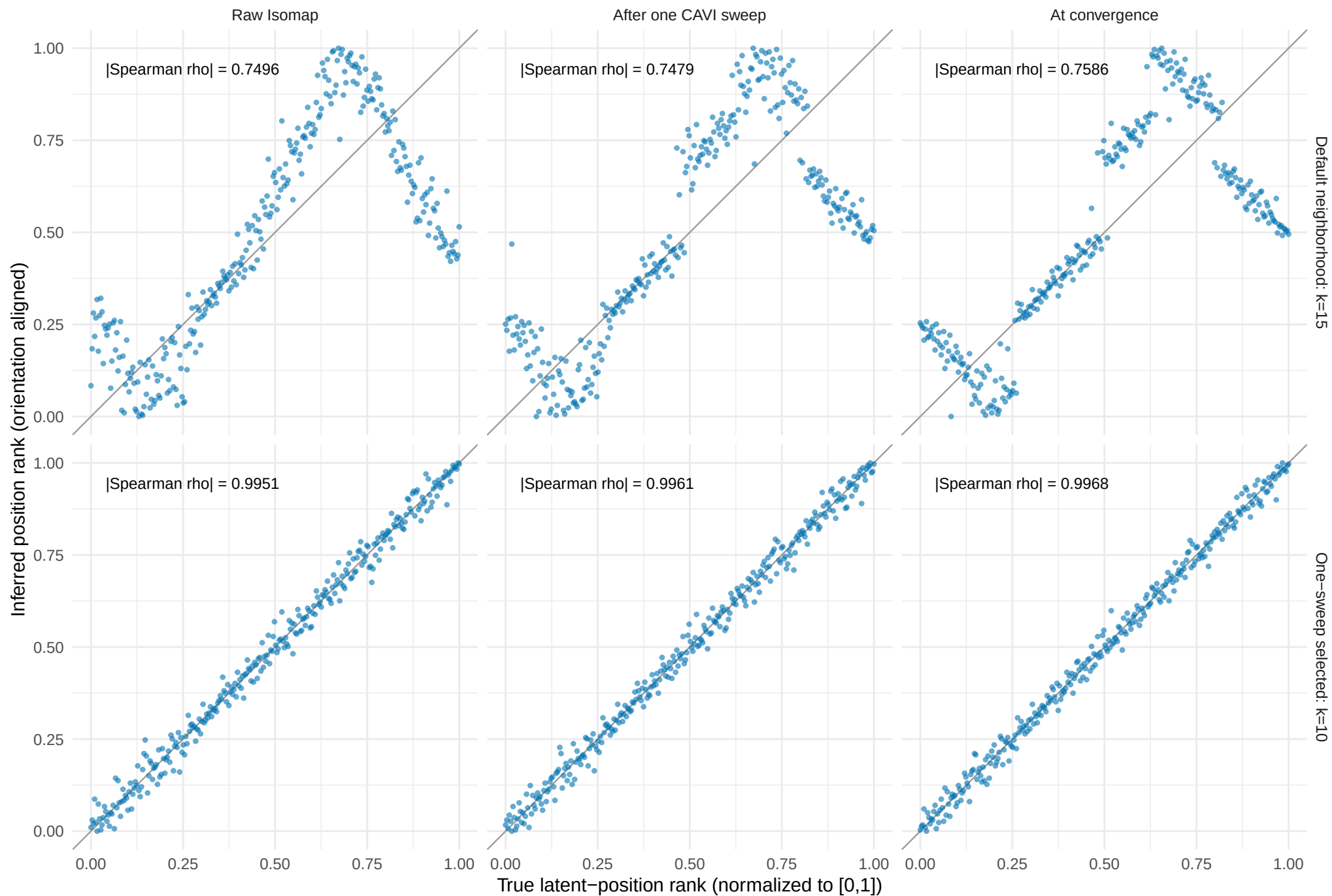
Figure 2. True and inferred normalized sample ranks for the k=15 comparator and the start selected solely by one-sweep ELBO. Columns show raw Isomap, one CAVI sweep, and convergence. Global reversal is aligned using truth for display only; the gray diagonal is perfect rank recovery. All 300 observations are retained; no truth coordinates enter fitting or ELBO selection.
