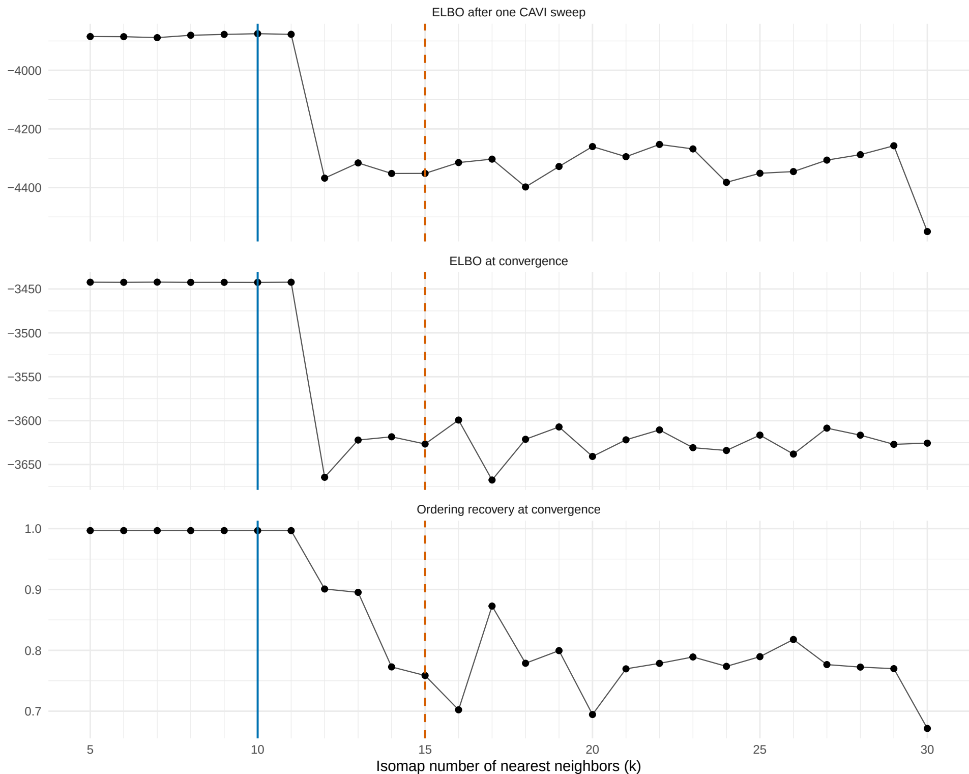
Figure 1. Each point is a neighborhood on the same 300-by-12 observation matrix. ELBO is compared within each fitting stage; higher values are preferred. Recovery is absolute Spearman correlation with true positions. Orange dashed line: k=15 comparator; blue solid line: one-sweep selection.
