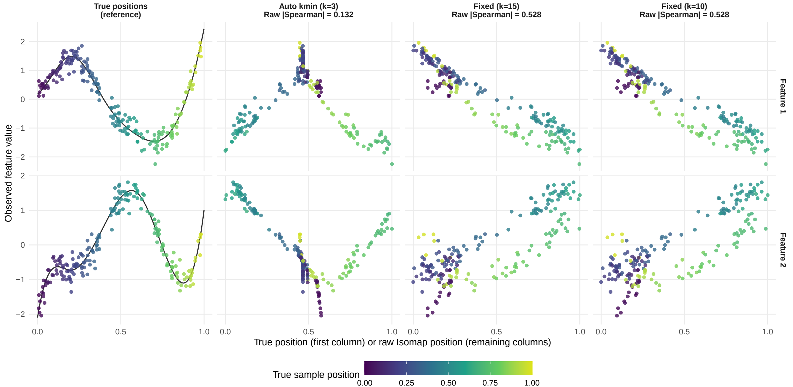
Figure 2. Each row shows one observed feature versus true positions or saved raw Isomap positions. The true-position column overlays the noiseless generating trajectory. Raw coordinates are before quantile binning and MPCurve optimization, scaled to [0,1] by the initializer. A global reflection, if needed, makes rank correlation positive for display; no rank transformation or nonlinear alignment is applied.
