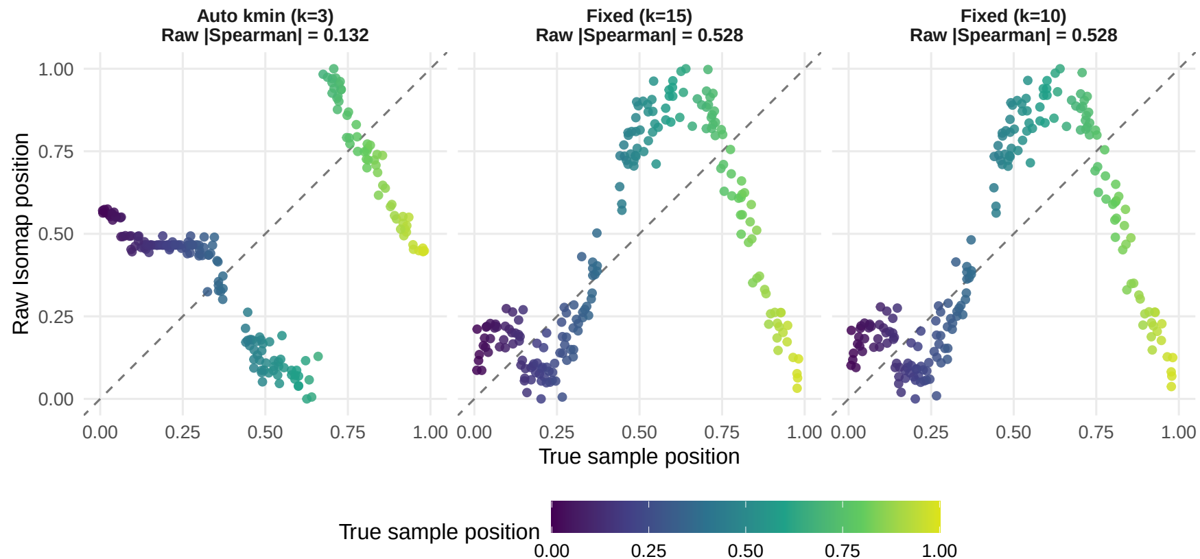
Figure 3. Saved initial Isomap coordinates against true positions for automatic kmin, k=15, and k=10. A global reflection allows ordering reversal for display. The dashed diagonal marks equal coordinates; Spearman assesses rank agreement rather than distance from that diagonal. Colors identify true positions.
