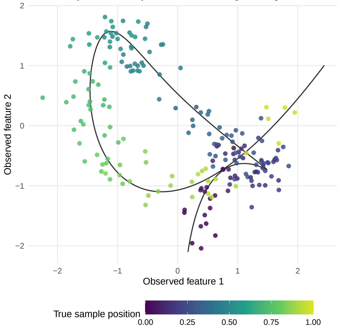
Figure 1. Two observed features for the selected N=200 , P=2 dataset. Colors identify true positions along the shared generating curve; the black line traces that curve in increasing true-position order. Independent observation-noise SD is 0.25.
