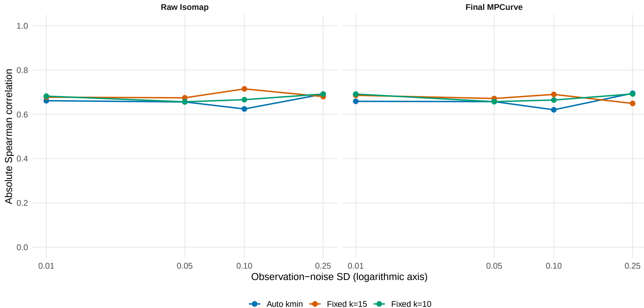
Figure 1. Raw Isomap and final MPCurve recovery at SD=0.25, 0.10, 0.05 , and 0.01 . Only error amplitude changes. Absolute Spearman allows global reversal. The original SD=0.25 fits are reused; all reduced-noise settings use the same frozen package and fitting controls. One fixed case; no uncertainty intervals.
