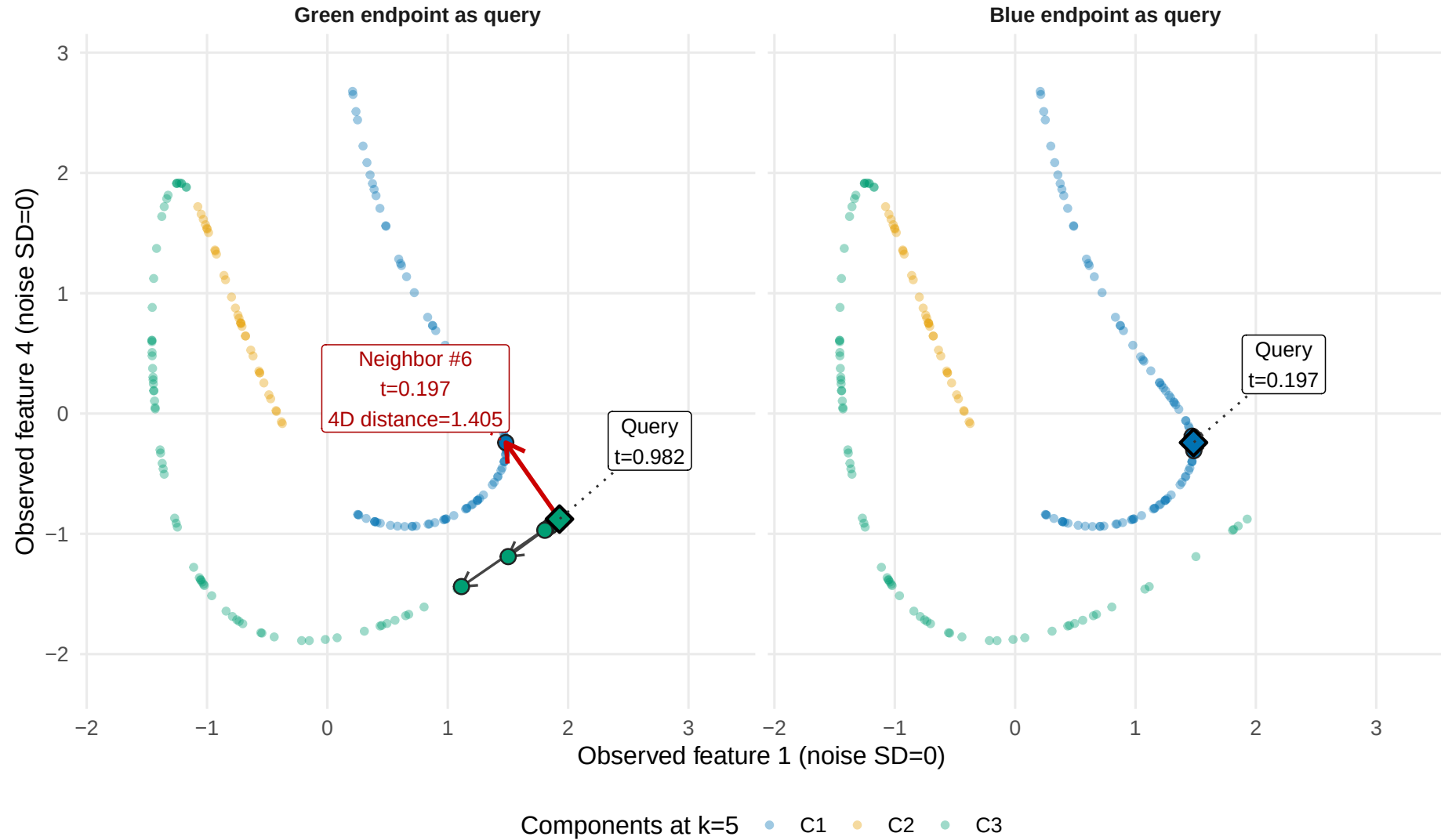
Figure 4. Six nearest neighbors of each endpoint of the noiseless shortcut, computed from all four features. Black diamonds mark queries; arrows point from each query to its selected neighbors. The red arrow is selected by the green endpoint only. Background colors are the k=5 components from Figure 3. The green endpoint has five green neighbors before this blue sixth neighbor; the blue endpoint selects six blue neighbors and ranks the green endpoint 64th. Axes are features 1 and 4.
