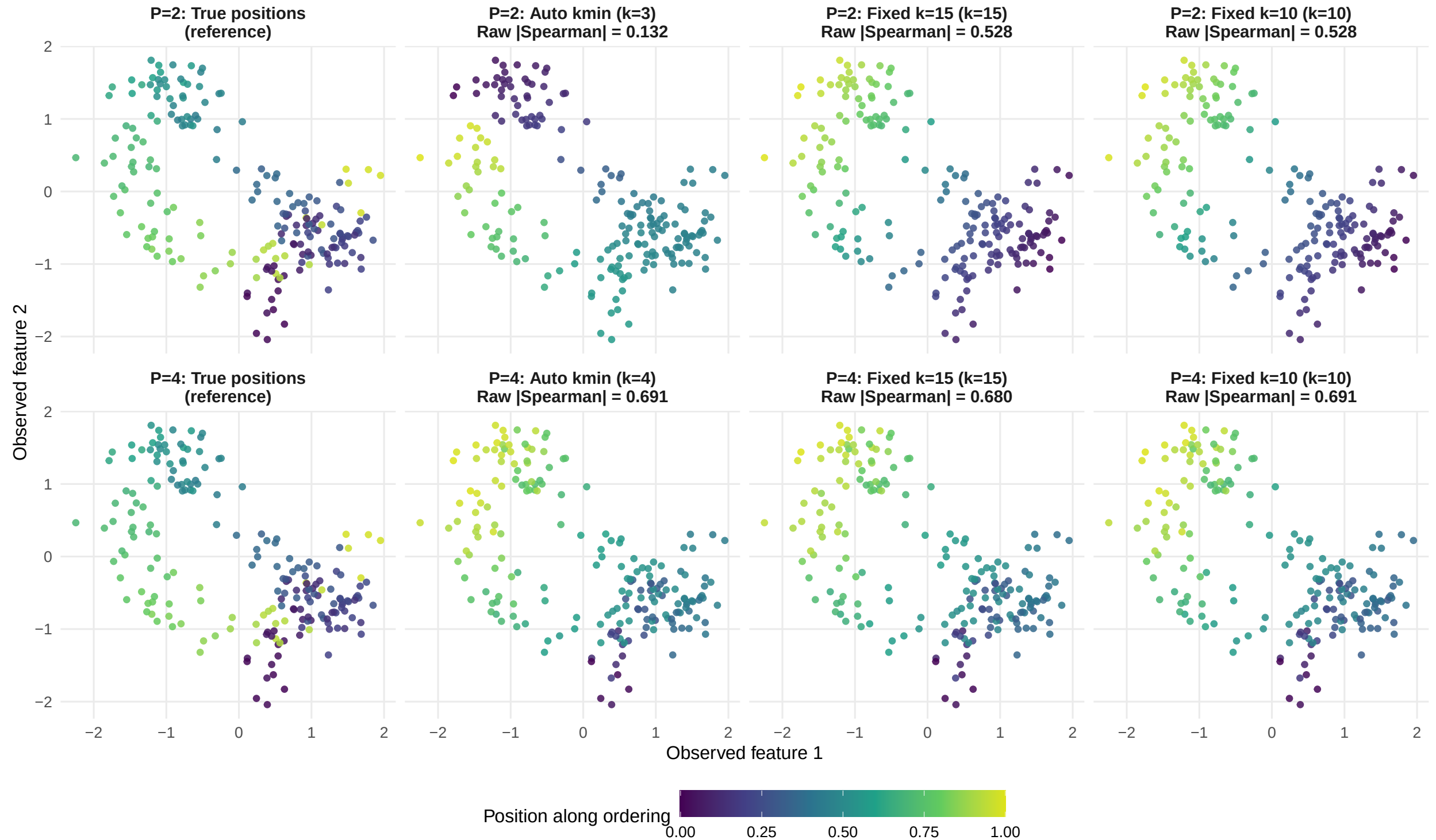
Figure 2. Identical observed feature-1/feature-2 scatter in all eight panels. Colors show true positions or raw Isomap positions computed from the indicated total number of features, before MPCurve fitting. Only a global reflection makes signed rank correlation positive for display. All panels share axes and color limits. The case was chosen in the preceding P=2 diagnostic; no new case selection uses P=4 outcomes.
