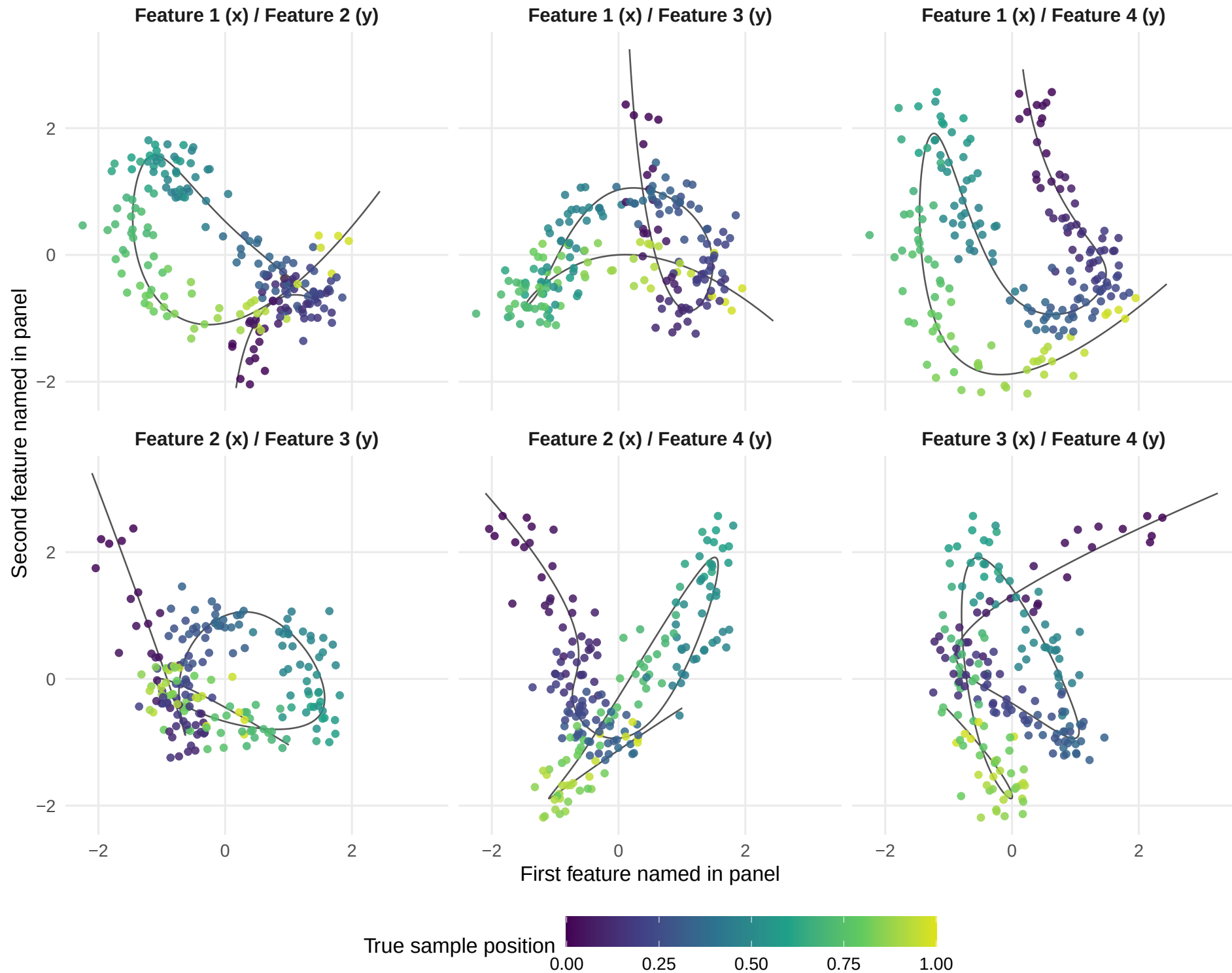
Figure 3. All six pairwise projections of the same P=4 observations, with named horizontal/vertical features. The first two features and their noise are unchanged from P=2 . The added independent trajectories provide extra joint information even when individual two-feature projections have crossings or close approaches. Axes share observed-feature units.
