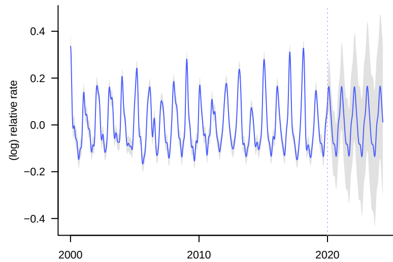
(c): Seasonal
