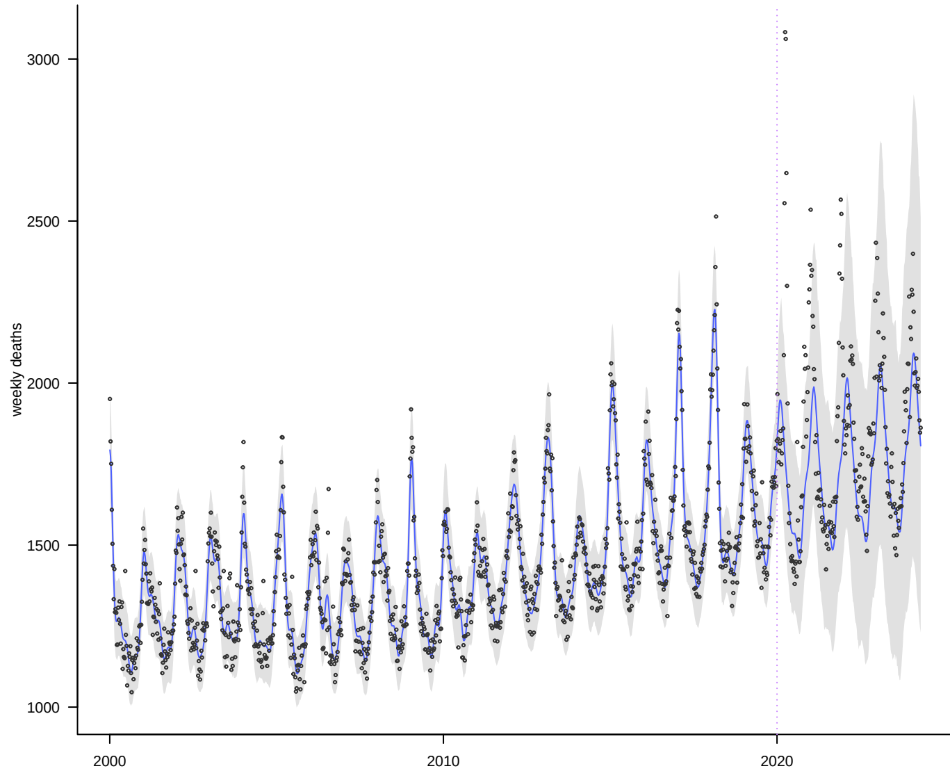
(a): Overall
