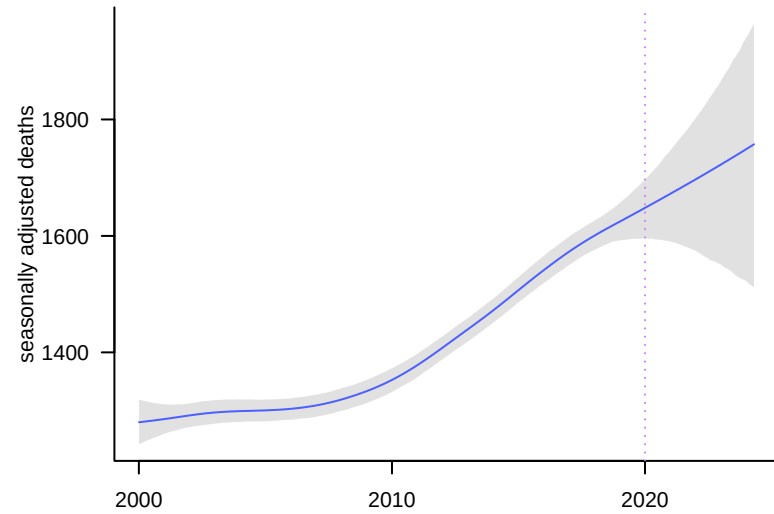
(b): Trend
