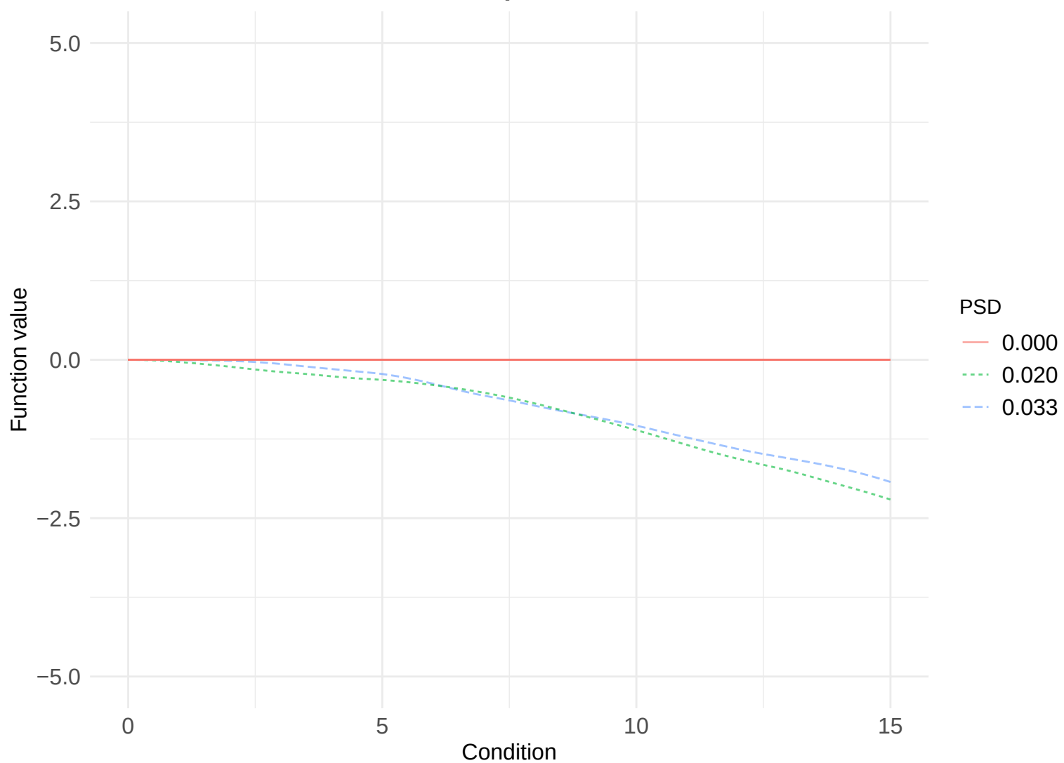
Linear baseline model: after BF update
