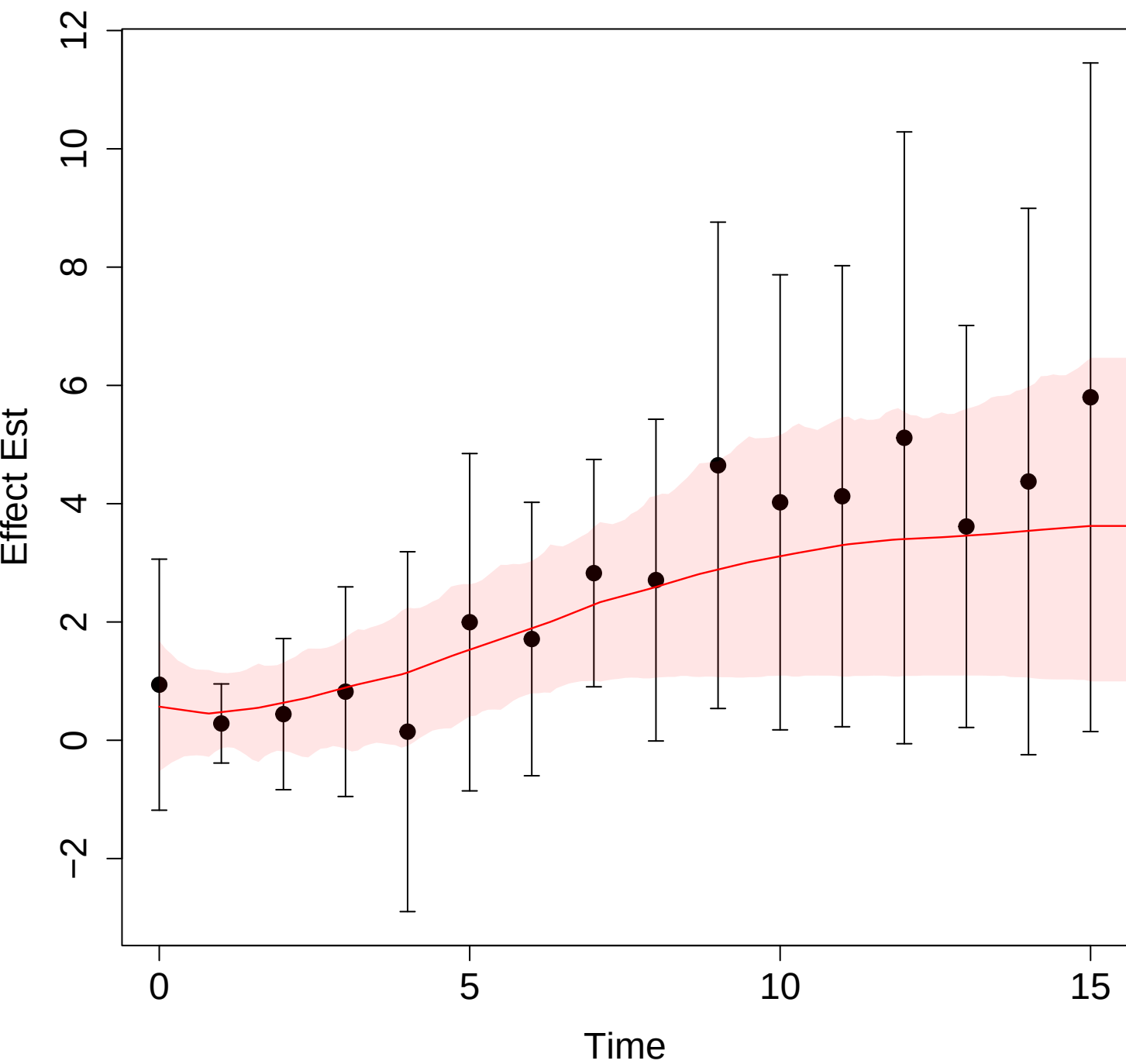
Penalize toward constant model
