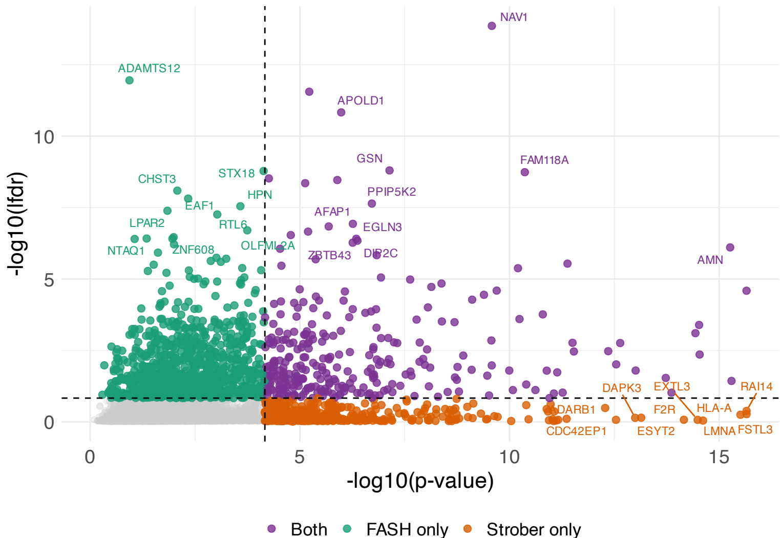
Scatterplot of lfr (FASH) vs p-values (Strober Quadratic)
