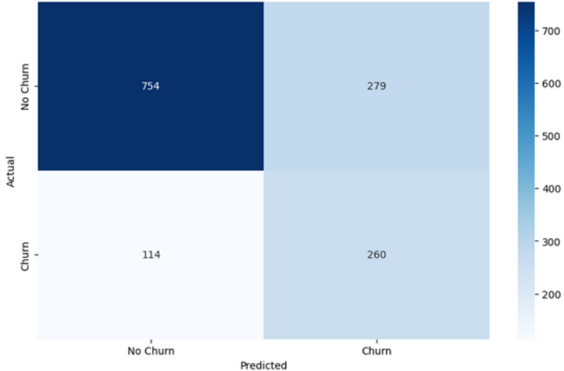
Confusion Matrix
