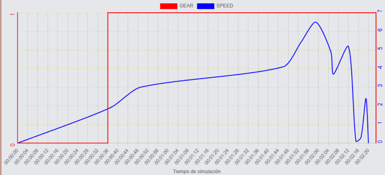
GRAPH B/W SPEED (In Km/h) vs GEAR (1:Forward 0:Neutral -1:Reverse)
