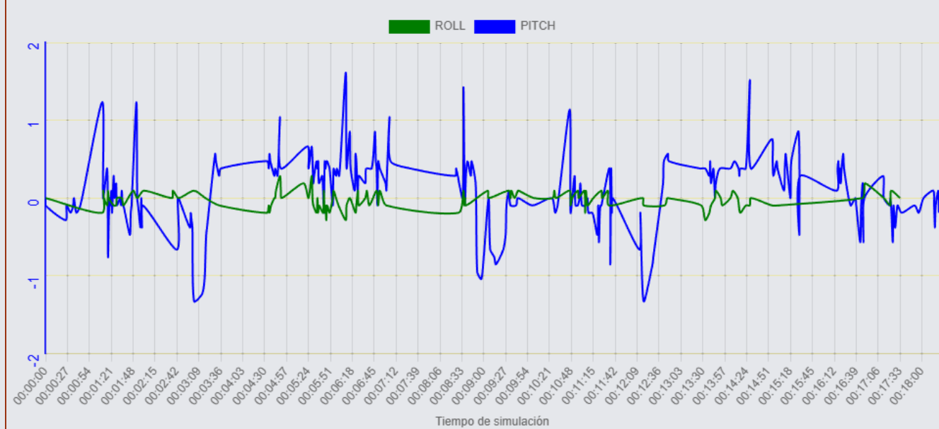
GRAPH B/W ROLL AND PITCH IN DEG
