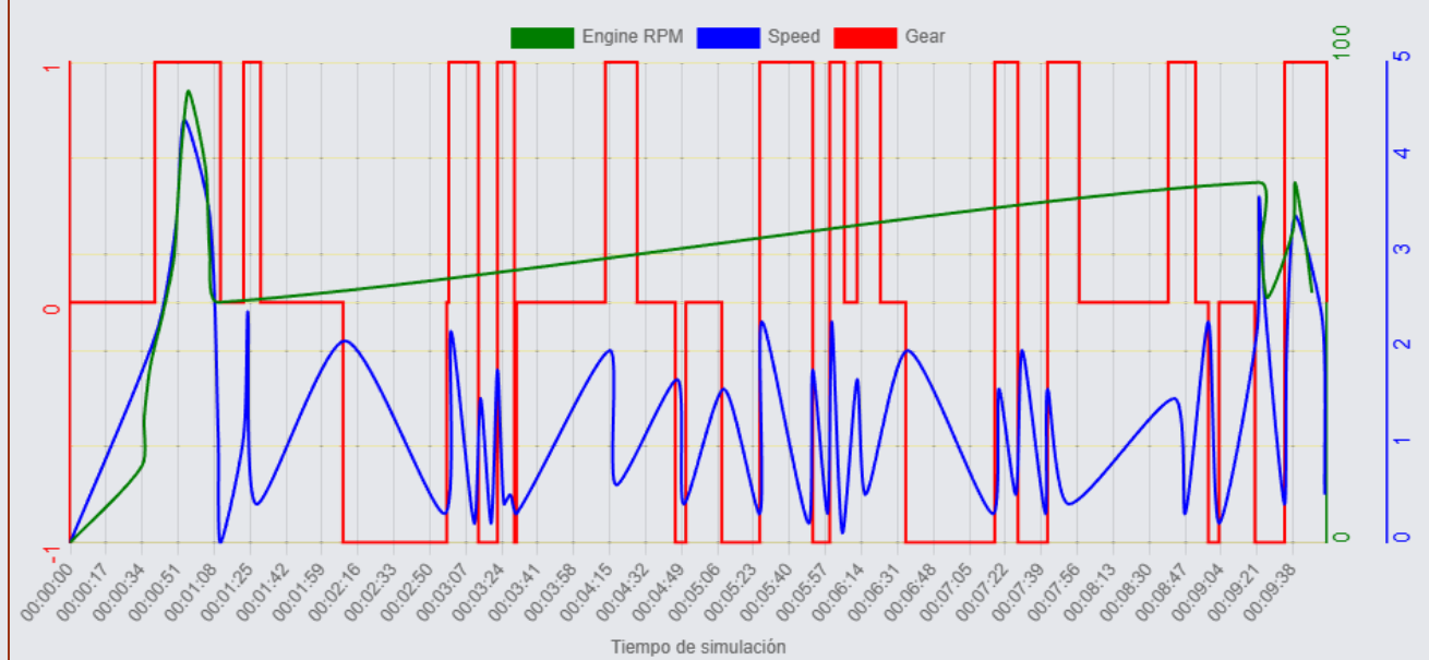
Graph B/W Engine RPM (0=Min 1050=Max), Speed (km/h) and Gear (1=Forward 0=Neutral -1=Reverse)
