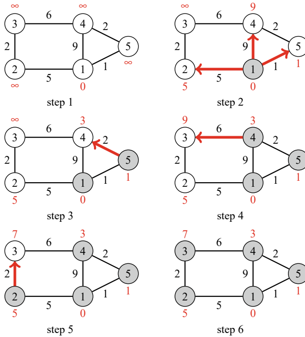
Fig. 7.20 Dijkstra's algorithm
