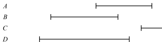
Fig. 4.7 An instance of the restaurant problem
