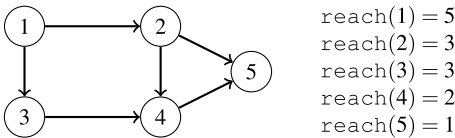
Fig. 8.2 A graph and its \text{reach} values. For example, \text{reach}(2) = 3 , because nodes 2, 4 and 5 can be reached from node 2
