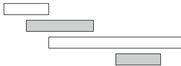
Fig. 4.9 An instance of the scheduling problem and an optimal solution with two events
