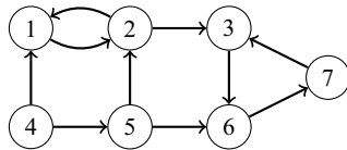
Fig. 12.3 The processing order of the nodes
