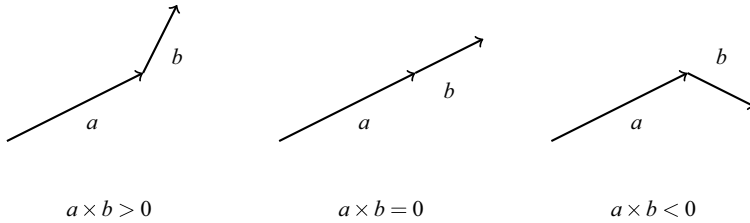
Fig. 13.2 The interpretation of cross products
