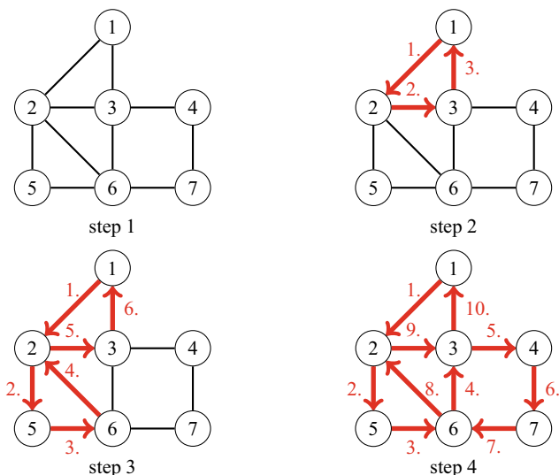
Fig. 12.12 Hierholzer's algorithm
