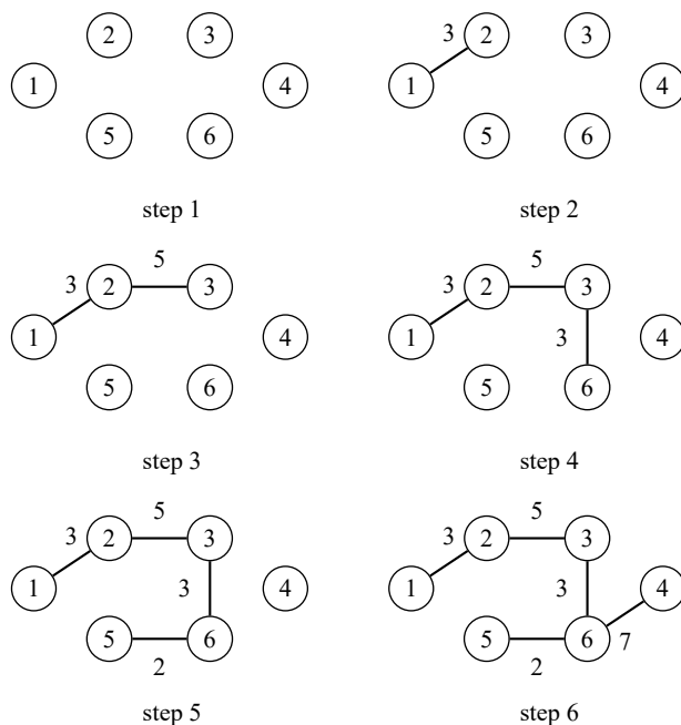
Fig. 7.43 Prim's algorithm
