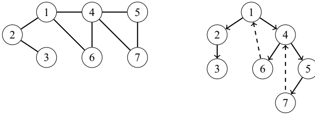
Fig. 12.39 A graph and its depth-first search tree
