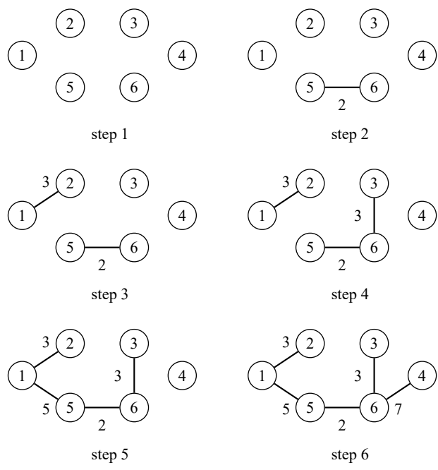
Fig. 7.38 Kruskal's algorithm
