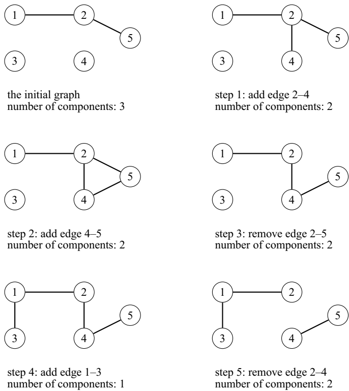
Fig. 15.35 The dynamic connectivity problem
