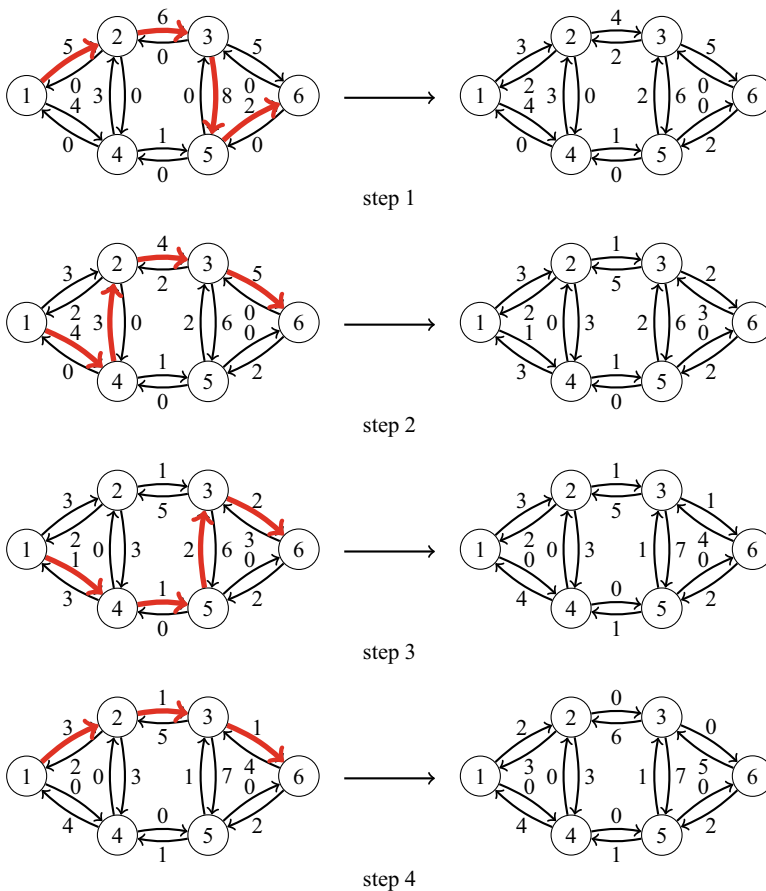
Fig. 12.21 The Ford-Fulkerson algorithm
