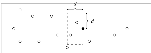
Fig. 13.20 The region where the closest point must lie
