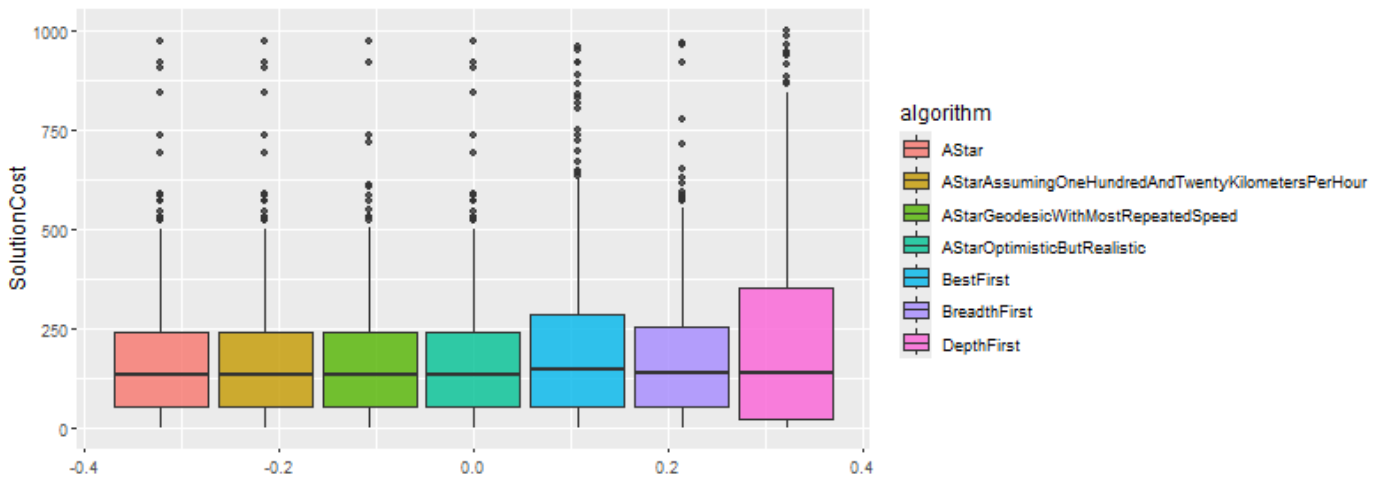
Figure 3: Boxplot on different solution costs by each search strategy.
