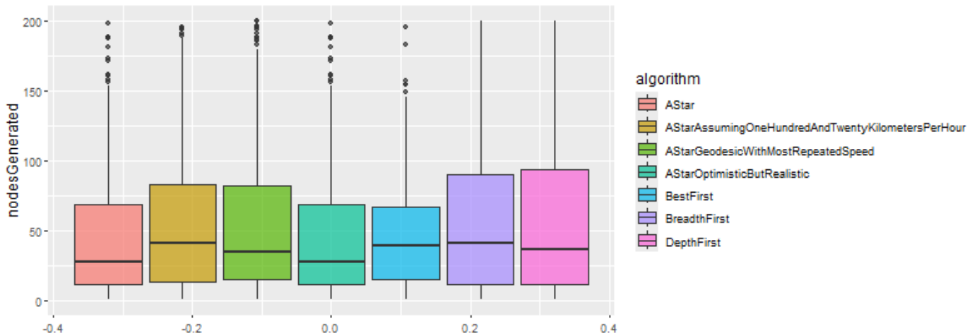
Figure 1: Graphic showing the nodes generated of each strategy.
