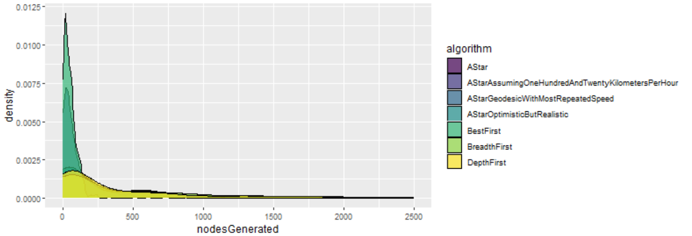
Figure 4: Density graph on the nodes generated by each strategy.
