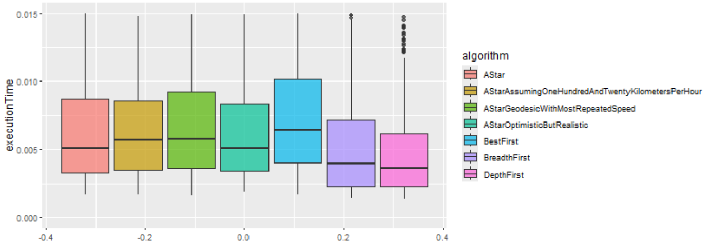
Figure 2: Graphic showing the different execution times of different strategies.
