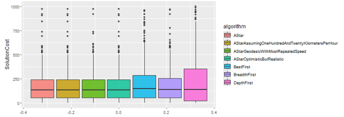
Figure 8: Boxplot on different solution costs by each search strategy.
