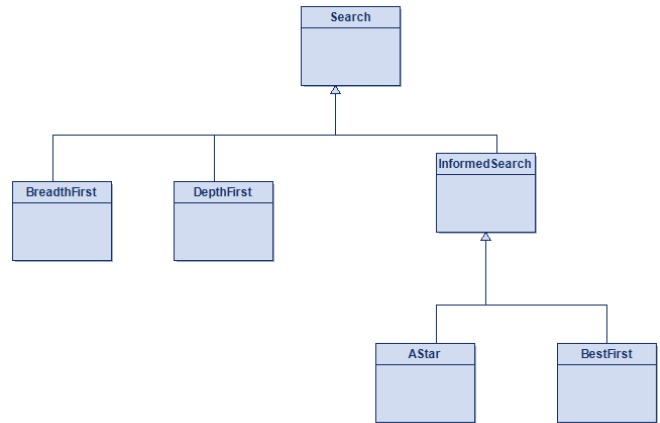
Figure 1: Class Diagram showing Inheritance.
