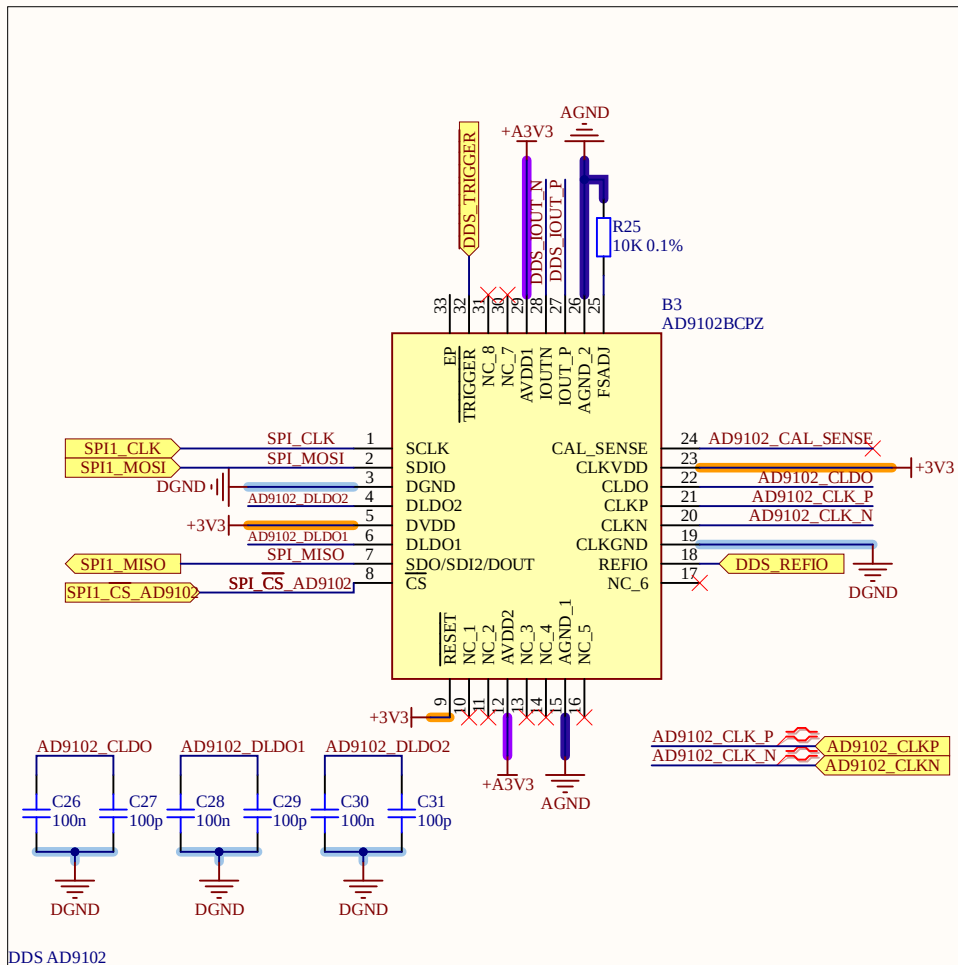
DDS AD9102
