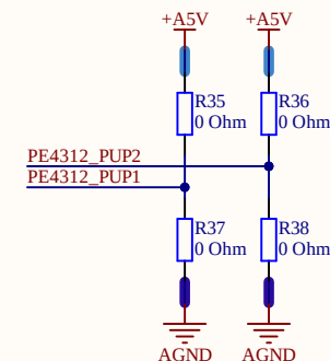
CONFIGURAR PULL UPS
