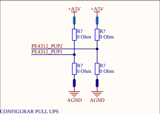
CONFIGURAR PULL UPS
