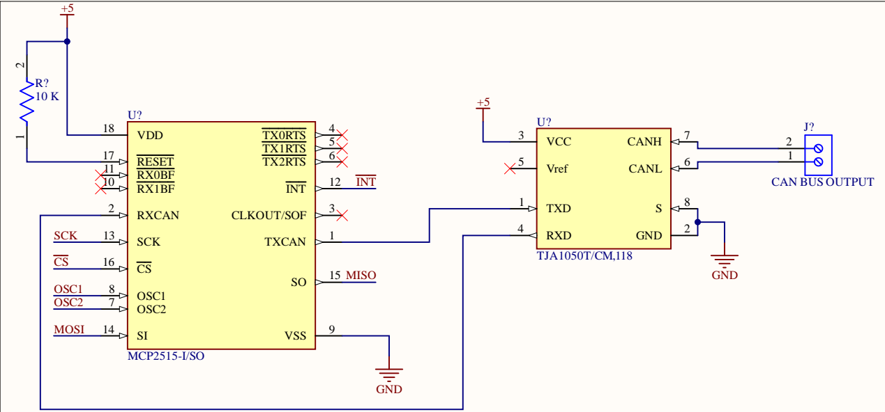
CONTROLADOR CAN - TRANSCEPTOR
