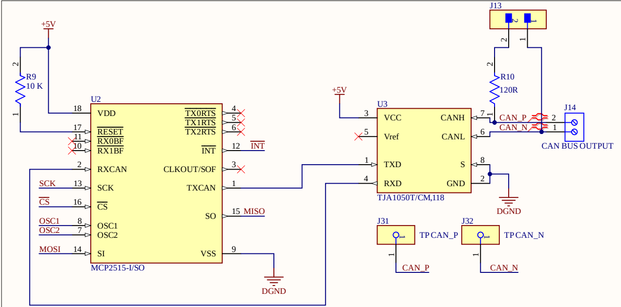
CONTROLADOR CAN - TRANSCEPTOR
