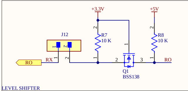
LEVEL SHIFTER
