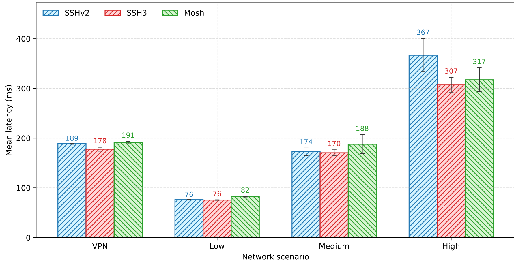
W1: Mean Command Latency by Scenario
