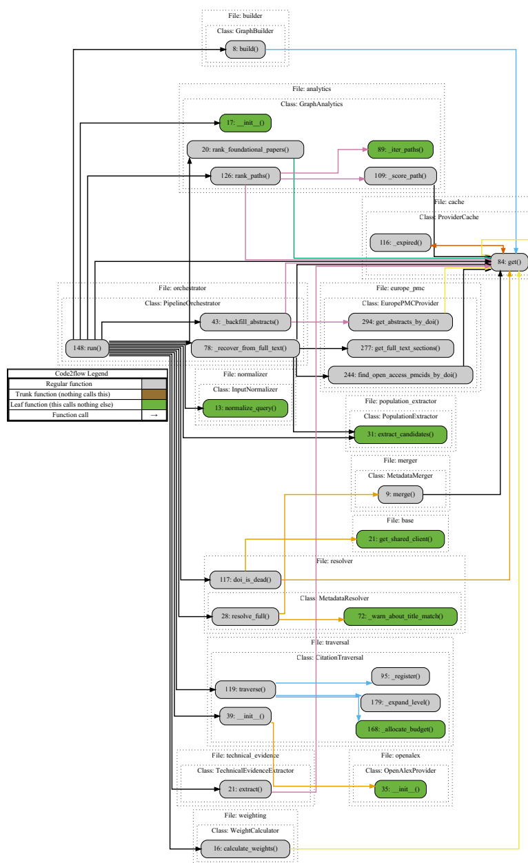
Figure 5.1 Calls made by PipelineOrchestrator.run() , traced by code2flow over the source and cut two levels below the entry point. Node labels carry the line number the function is defined at, so the figure doubles as an index into the source. Dotted boxes are files and classes, and green nodes call nothing further within the project. run() sits at the left, the stages it calls form the middle column, and the functions those stages call in turn sit at the right.
