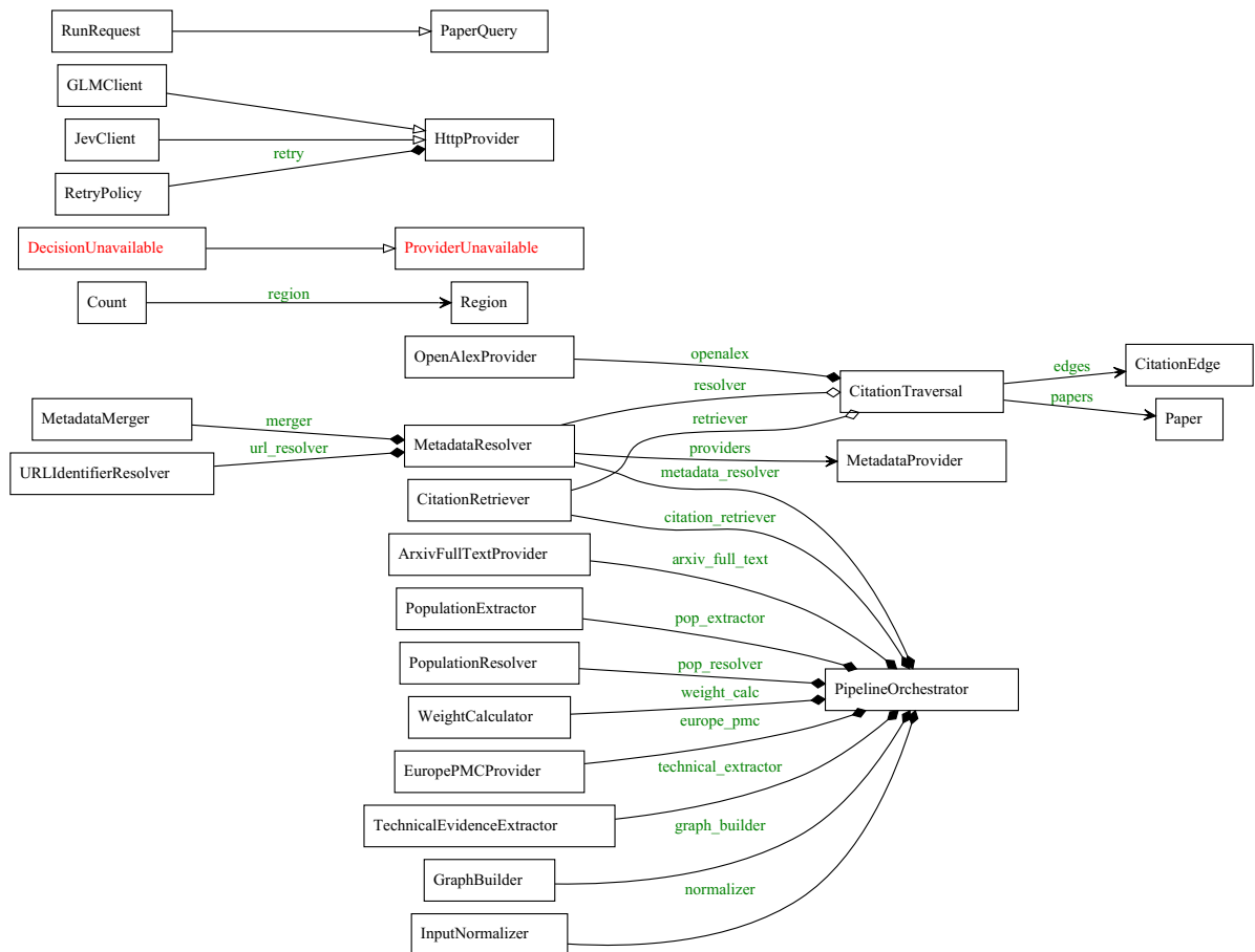
Figure 4.2 Object composition among the classes that participate in a relationship, from pyreverse with the 31 unrelated classes removed. PipelineOrchestrator composes ten collaborators, the stage modules and the two providers it calls directly; edge labels are the attribute names the orchestrator stores them under.
