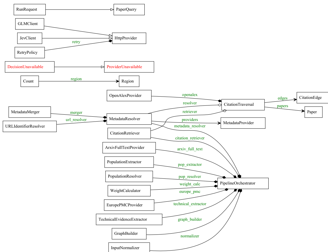
Figure 4.2 Object composition among the classes that participate in a relationship, from pyreverse with the 31 unrelated classes removed. PipelineOrchestrator composes ten collaborators, the stage modules and the two providers it calls directly; edge labels are the attribute names the orchestrator stores them under.
