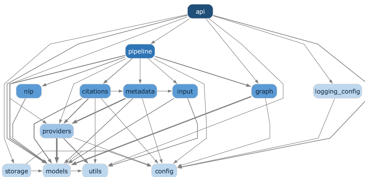
Figure 4.1 Inter-package dependencies, produced by running pyreverse over src/citegraph and collapsing its 46 module nodes to the 13 packages they belong to. Each arrow stands for one or more imports and is drawn thicker the more imports it carries. The heaviest arrows run downward into models , which holds the Pydantic types every other package constructs.
