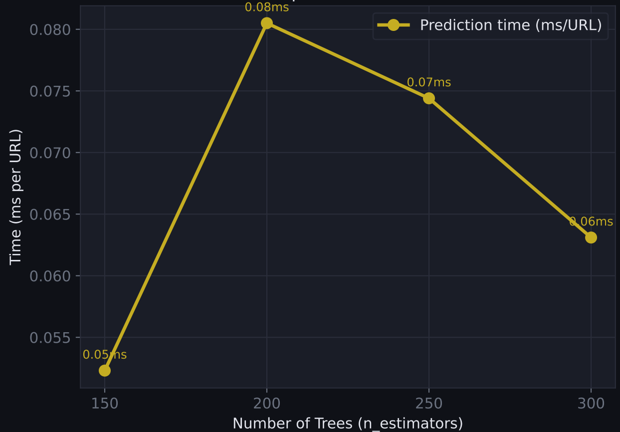
Prediction Speed vs Number of Trees
