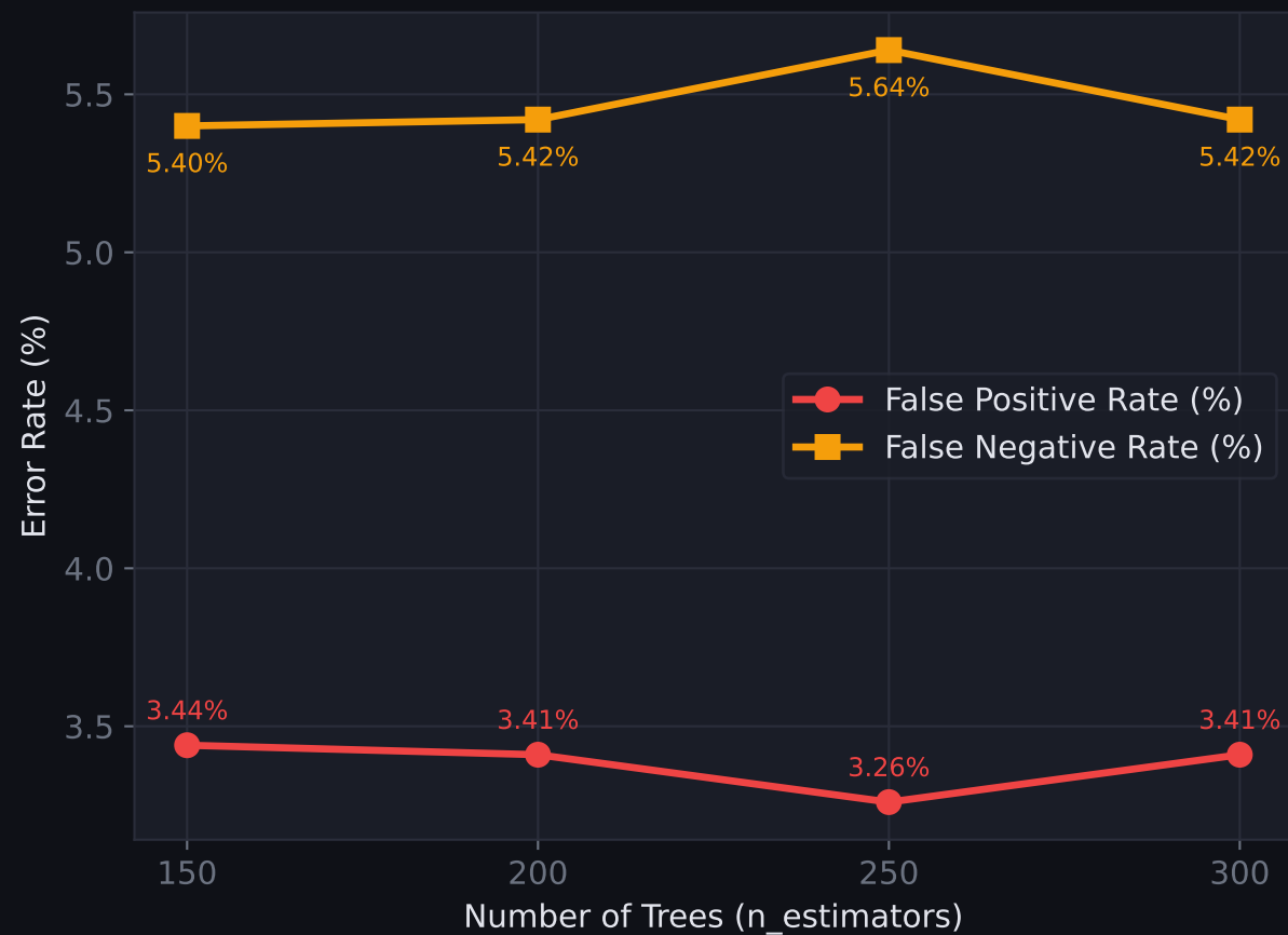
FPR &amp; FNR vs Number of Trees
