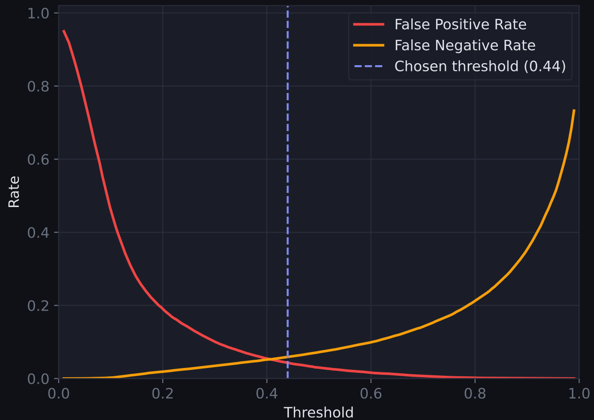
FPR / FNR vs Threshold
