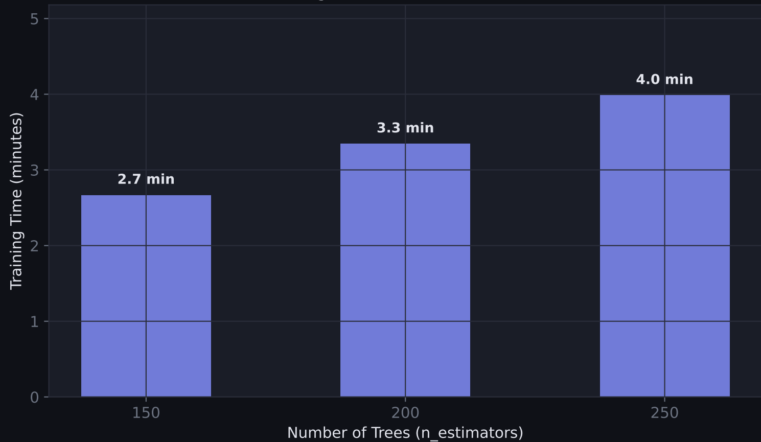
Training Time vs Number of Trees
