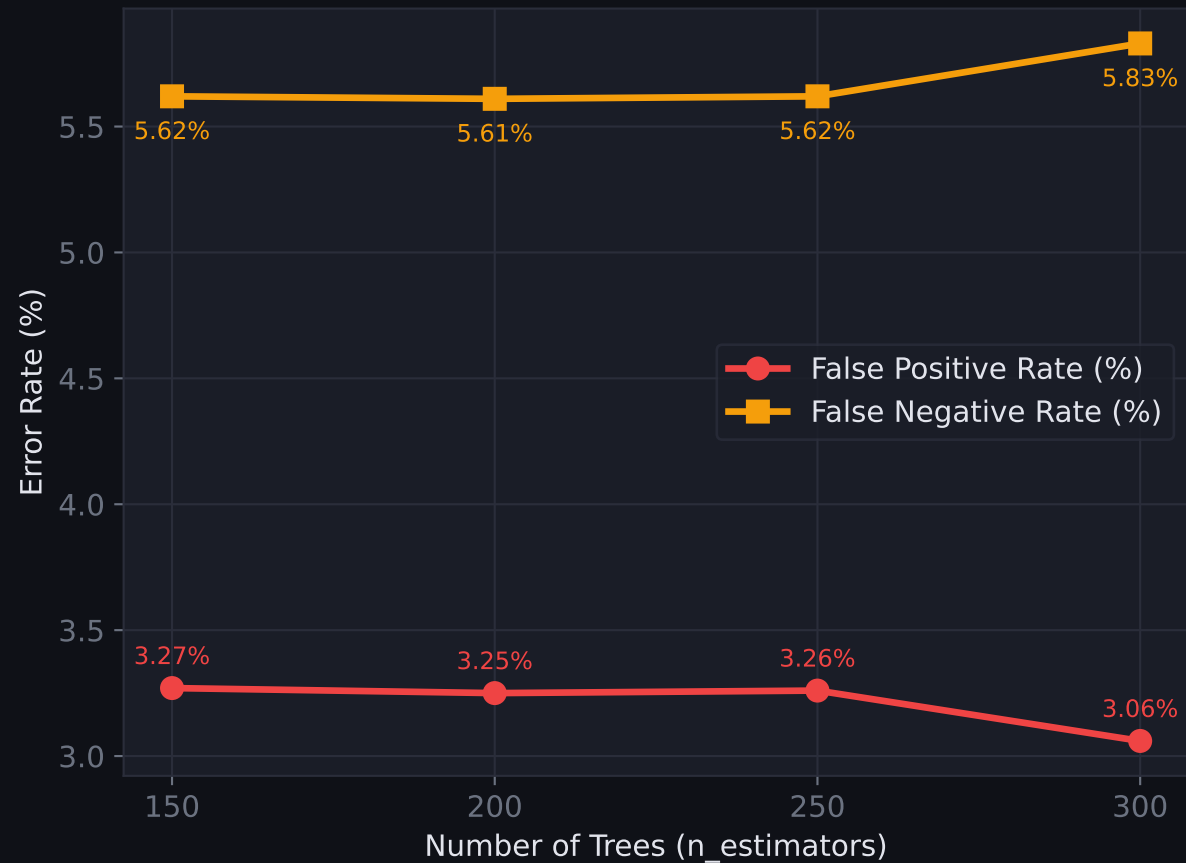
FPR &amp; FNR vs Number of Trees
