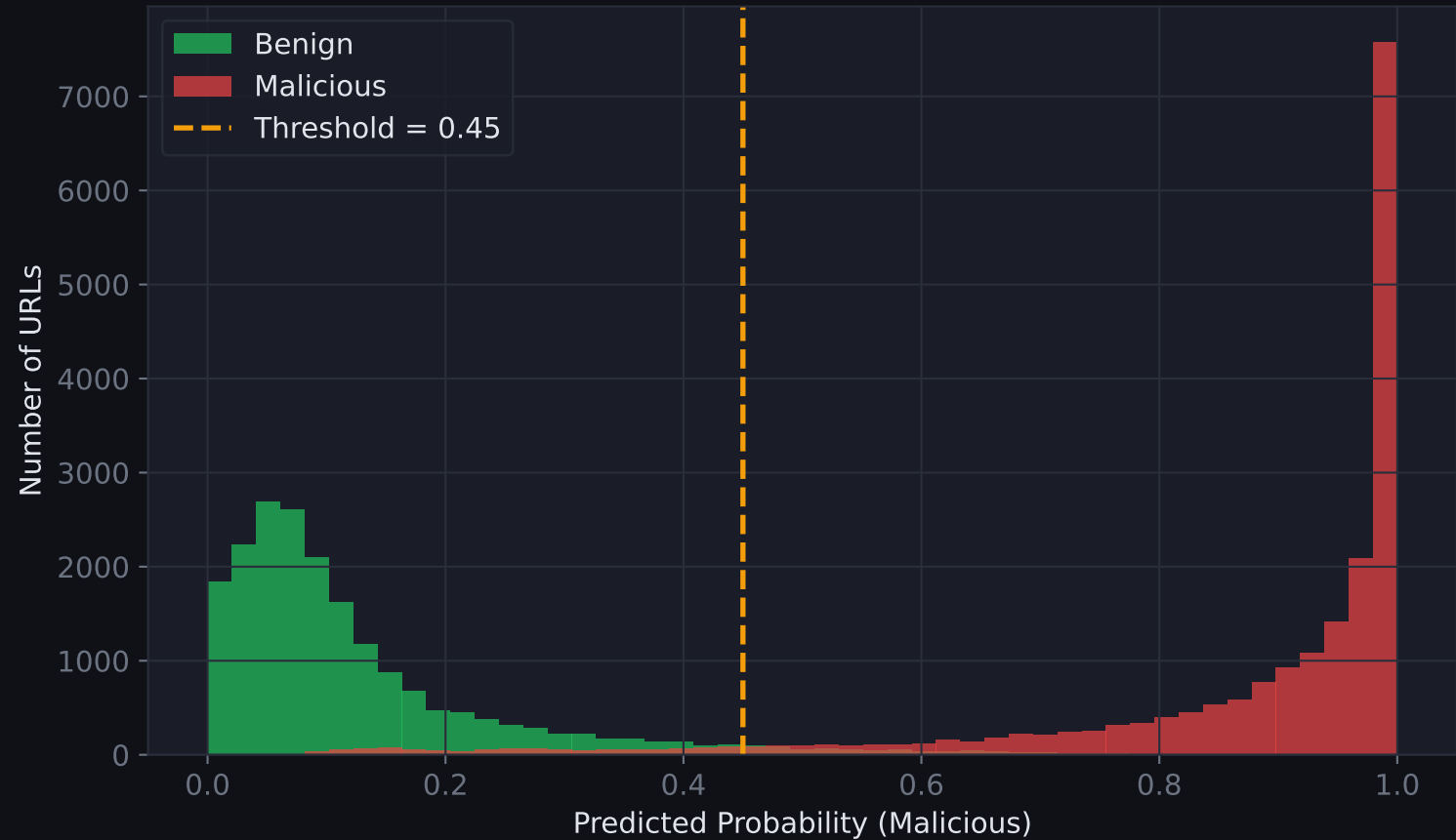
Confidence Score Distribution
