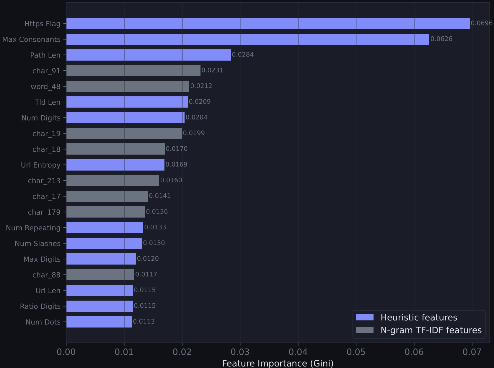
Top 20 Feature Importances
