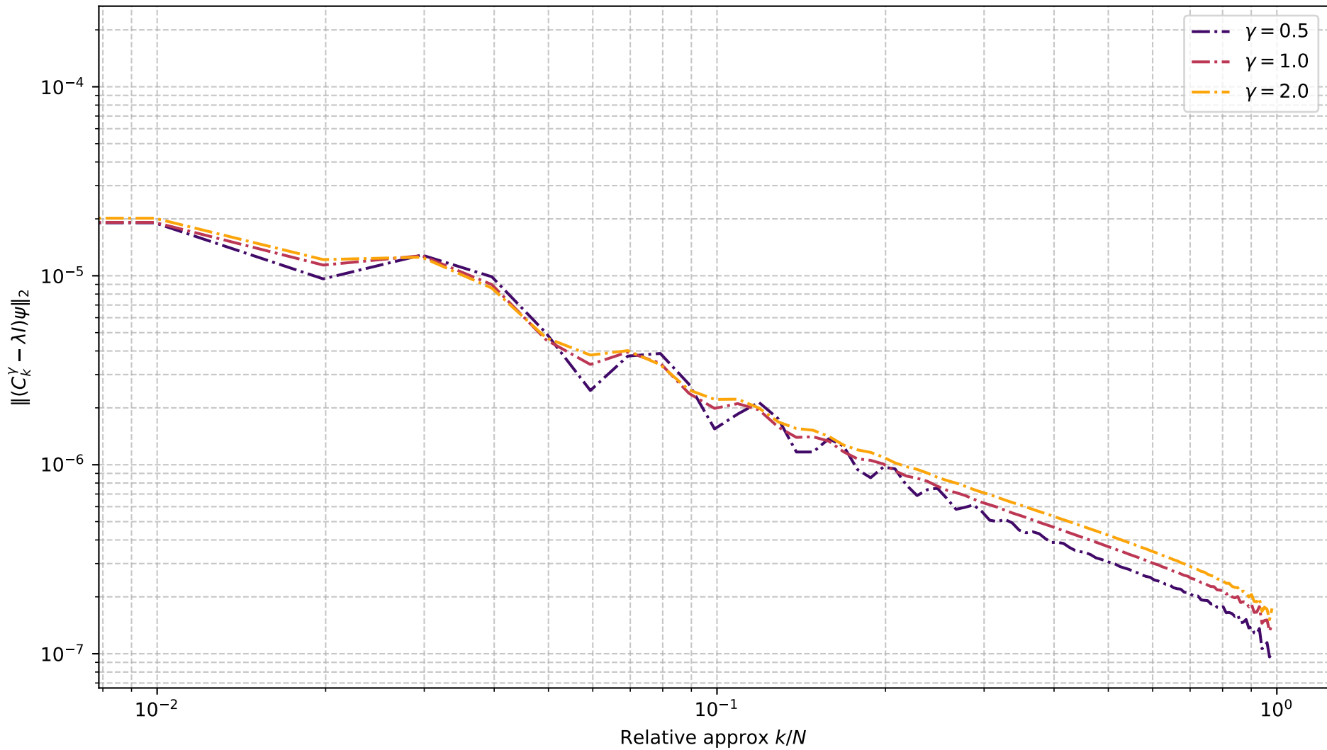
k-order approximation eigen problem relative error, N = 101 , R = 0.2 , \psi = \psi_{75}
