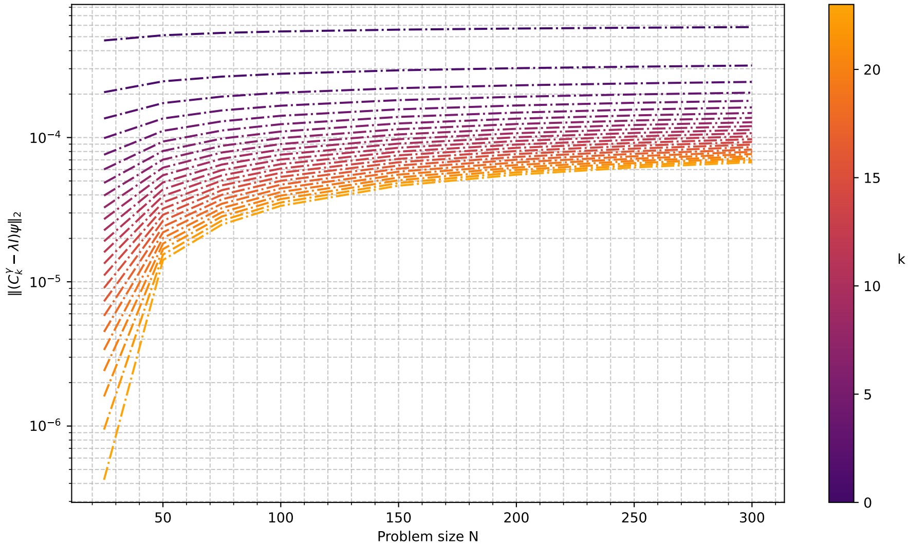
k-order approximation eigen problem error, R = 0.2 , \gamma = 1 , \psi = \psi_1
