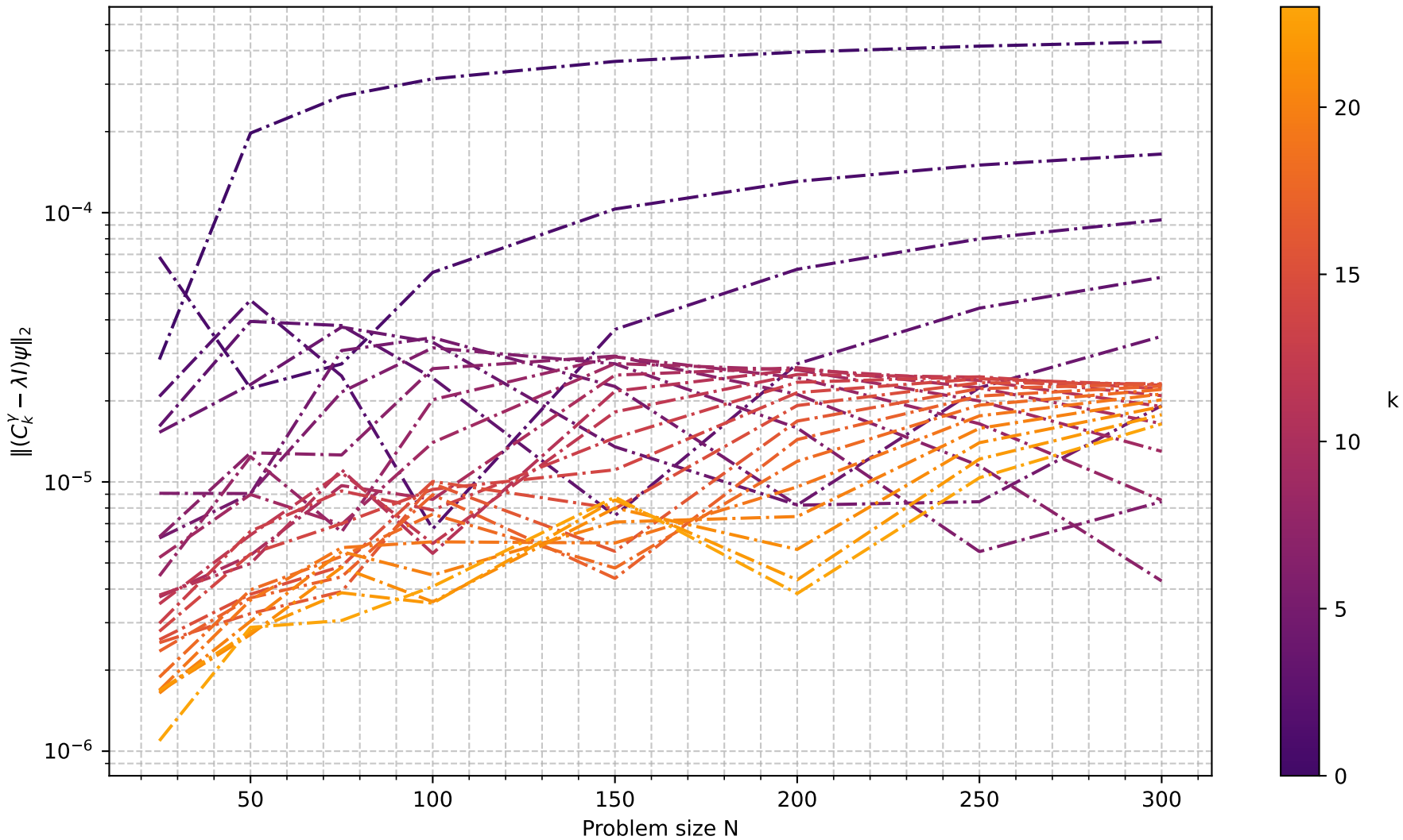
k-order approximation eigen problem error, R = 0.2 , \gamma = 1 , \psi = \psi_{10}
