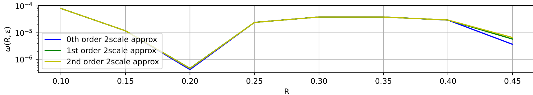
Error: \omega(R, \varepsilon) - (\omega_0(R) + (\varepsilon - \varepsilon_c)\omega_1(R) + (\varepsilon - \varepsilon_c)^2\omega_2(R)) , approx SI term
