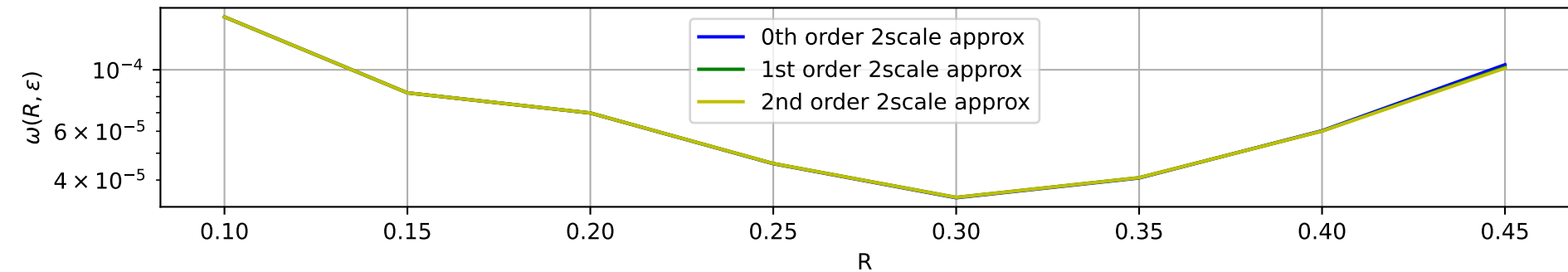
Error: \omega(R, \varepsilon) - (\omega_0(R) + (\varepsilon - \varepsilon_c)\omega_1(R) + (\varepsilon - \varepsilon_c)^2\omega_2(R)) , data SI term
