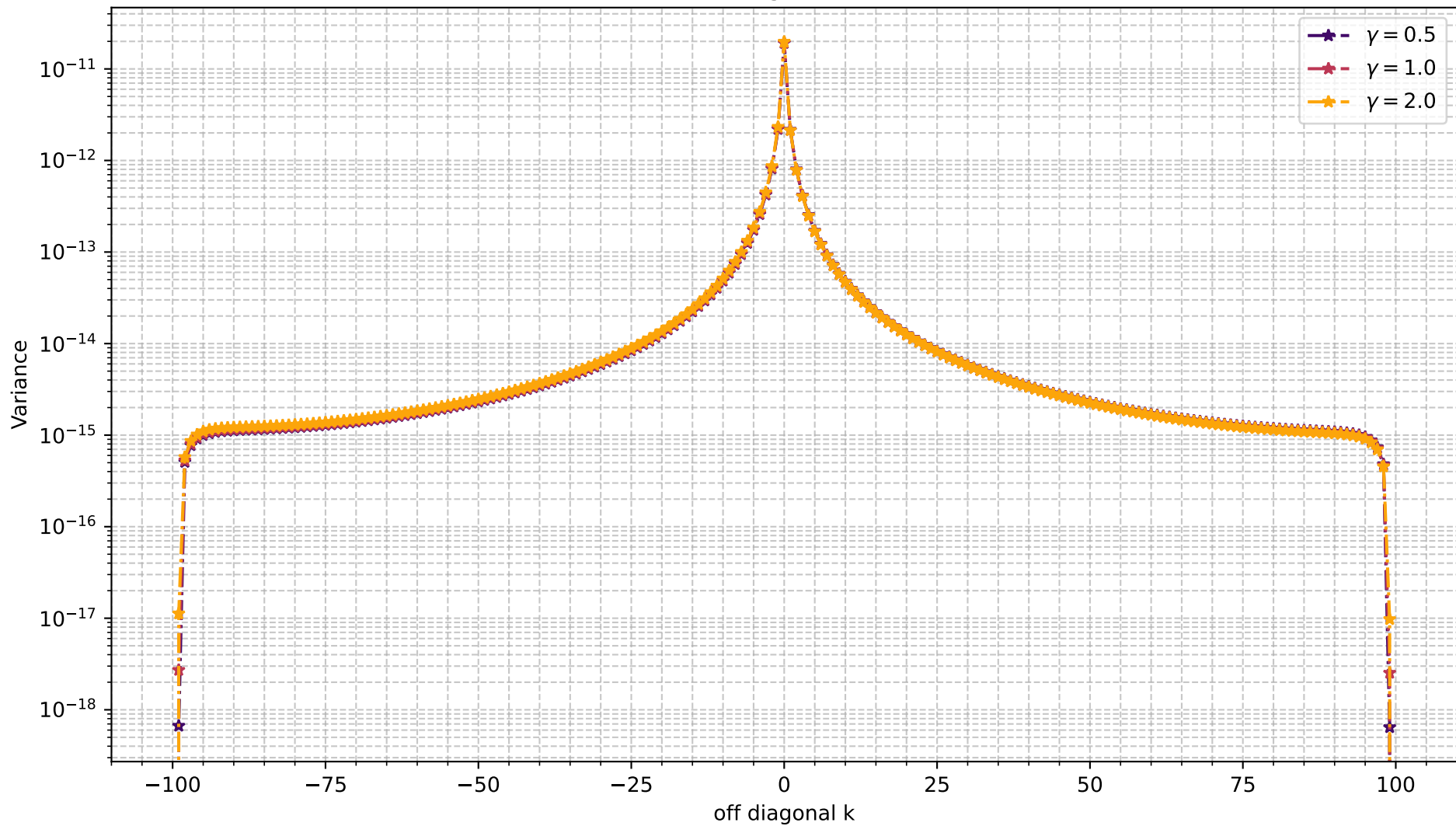
Variance of diagonal coefficients
