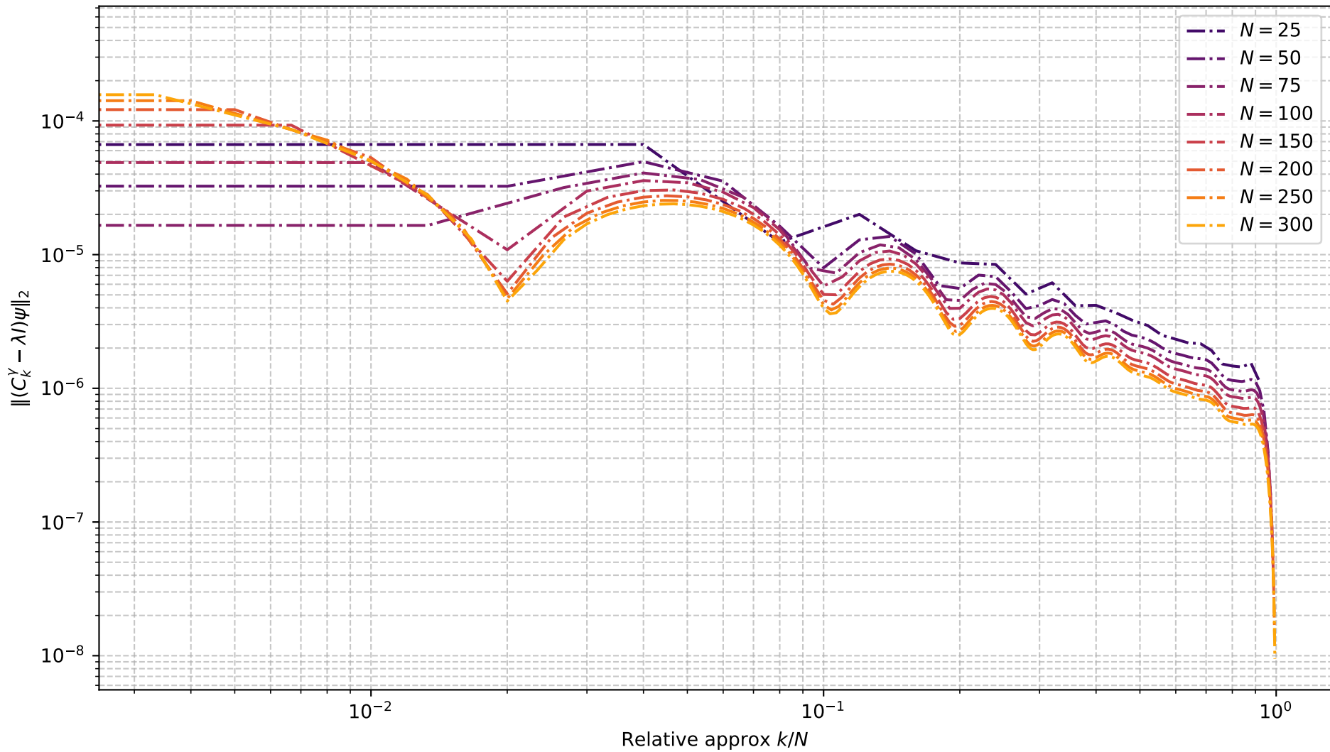
k-order approximation eigen problem relative error, \gamma = 1.0 , R = 0.2 , \psi = \psi_{10}
